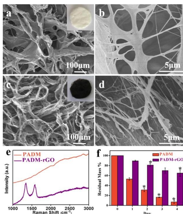
Figure 1. Characterization of the PADM and PADM-rGO scaffolds. SEM images of the topography of PADM (a, b) and PADM-rGO (c, d), the (a-inset) and (c-inset) are photographs of PADM and PADM-rGO with 8 mm diameter, respectively. (e) Raman spectra (514 nm) of the two scaffolds. (f) The percentage of residual mass of the PADM and PADM-rGO after enzymatic degradation at different time points. (* p \leq 0.05 , ** p \leq 0.01 , n = 3 )
