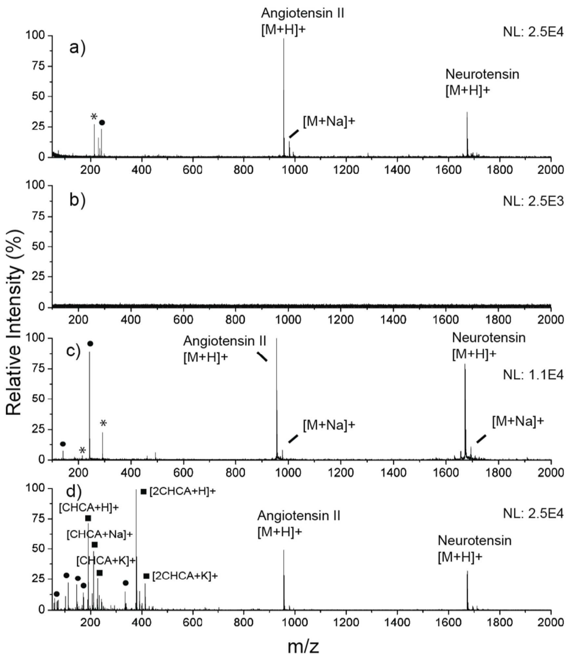
Figure 4. Ionization of [Sar 1 , Thr 8 ]-angiotensin II and neurotensin from various laser desorption/ionization substrates at laser fluence of 1900 a.u. S/N ratios are given for the angiotensin II [M+H] + peak. (a) Calcinated AuNP microarray (S/N = 72.0). (b) Bare AuNPs, with no silicate protection or calcination (no analyte signal). (c) Evaporated gold substrate with ca. 20 nm of silicate (S/N = 74.0). (d) CHCA matrix (S/N = 37.0).
