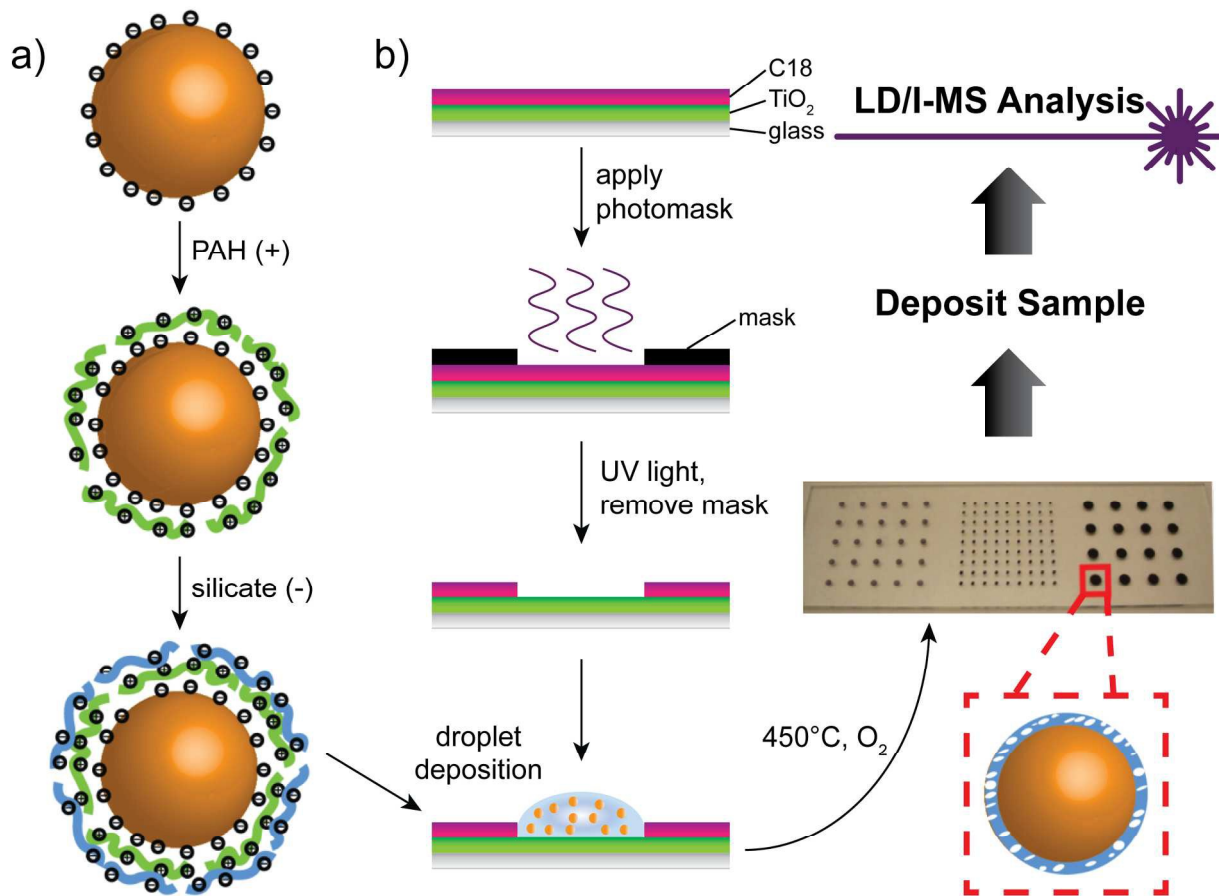
Figure 1. Fabrication of the calcinated AuNP array and analytical scheme. (a) Layer-by-layer modification of gold nanoparticle surface in solution. (b) Photocatalytic method for creating a hydrophilic spot pattern with hydrophobic surroundings on glass microscope slides.
