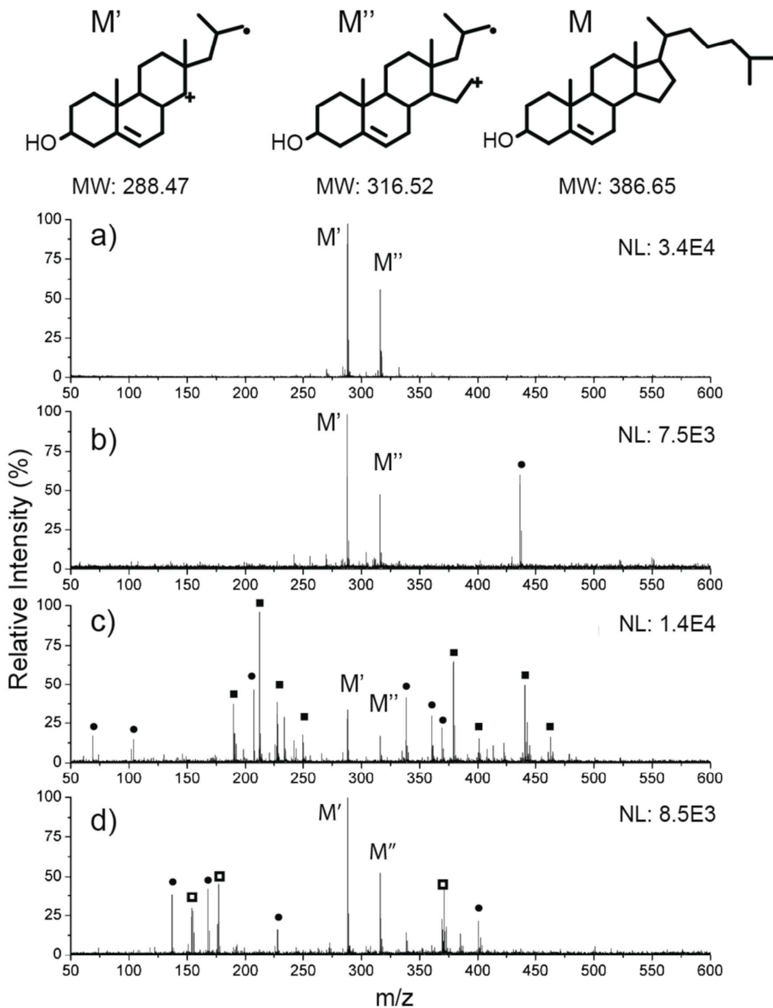
Figure 5. Ionization of cholesterol from various surfaces and matrices. S/N ratios are given for the M' peak. (a) Calcinated gold nanoparticle array (S/N = 70.0). (b) Uncalcinated AuNP-(PAH-silicate) 1 construct (S/N = 35.5). (c) CHCA matrix (S/N = 12.5). (d) DHB matrix (S/N = 36.0).
