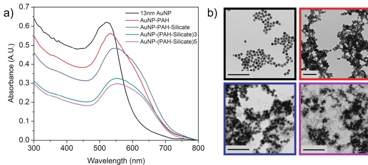
Figure 2. Layer-by-layer modification of gold nanoparticles. (a) Monitoring of polymer and silicate depositions using localized surface plasmon resonance absorbance bands. (b) Corresponding transmission electron micrographs. Scale bars represent 100 nm.
