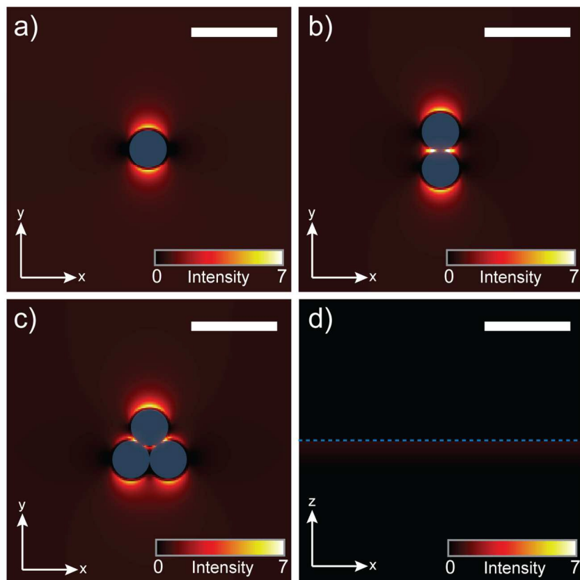
Figure 7. Numerical simulations of plasmonic fields induced by \lambda = 337 nm light source for different nanoscale geometries. Scale bars represent 30 nm and blue represents the gold surface. (a) Single gold nanoparticle. (b) Gold nanoparticle dimer. (c) Gold nanoparticle trimer. (d) Planar gold film.
