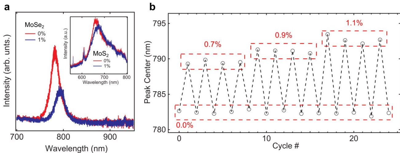
FIG. 2. (a) PL spectra for a single layer MoSe 2 flake at 0% and 1% strain. The inset shows the PL spectra for a single-layer MoS 2 flake at 0% and 1% strain. Note that the wavelength scale is the same width for both plots showing clearly the difference in the FWHM between the MoSe 2 PL peak and the MoS 2 PL peak. (b) Center of the PL peak for single-layer MoSe 2 as a function of strain for several straining cycles. PL shifts for strains up to 1.1% are reproducible using the simple clamp and bend apparatus in Figure 1(c).
