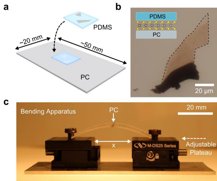
FIG. 1. (a) A viscoelastic (PDMS) stamp with exfoliated MoSe 2 is placed upside down onto a polycarbonate (PC) substrate to create a PC-MoSe 2 -PDMS stack. (b) Optical transmission image of a MoSe 2 flake sandwiched between PC and PDMS. The inset shows a cartoon of the sandwich for a single-layer flake. (c) Optical image of the apparatus used to bend the sandwich and apply strain to the MoSe 2 flake.
