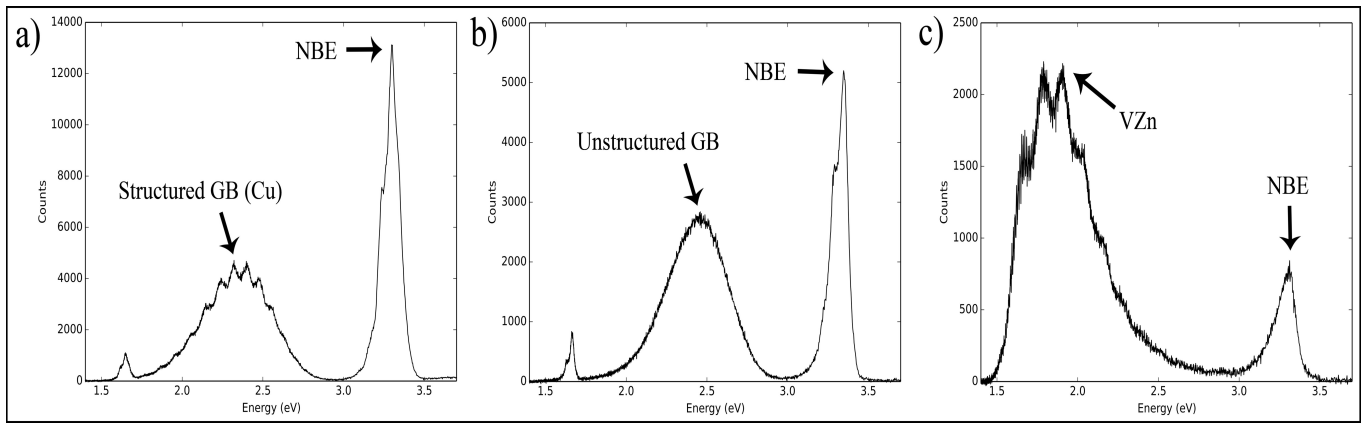
FIG. 3. a) CL spectrum from set A ( Cu_{Zn} ). b) CL spectrum from set B (UGB). c) CL spectrum from set C ( V_{Zn} ).
