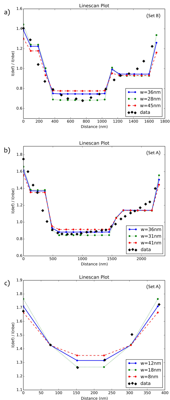
FIG. 4. DRCLS line-scan plots showing simulation's best fit (blue lines), error bounds (green & red lines), and measured data (black diamonds) for a) 1.7\mu\text{m} wire b) 2.2\mu\text{m} wire and c) 380\text{nm} wire. The segregation width ( w ) is included for each fit.
