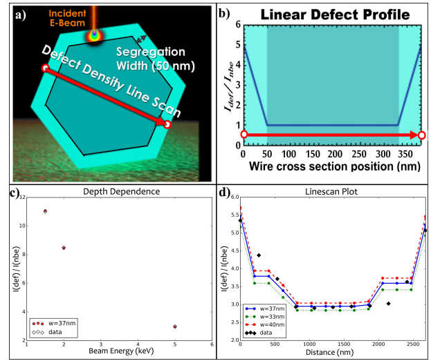
FIG. 2. a) Cross section view of ZnO wire showing how the defect line scan plot in (b) is mapped onto physical space. b) Illustration of how defects vary across a wire's cross section for a linear decay profile. c) Single spot depth dependence measurement on a ZnO wire's top face d) Corresponding 5 keV line-scan fit for wire from (c) (blue dots represent the best fit).
