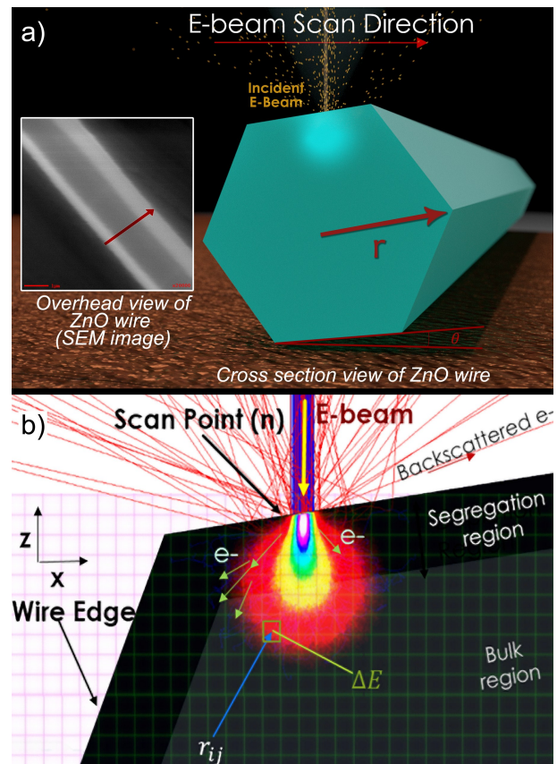
FIG. 1. a) Illustration showing the line-scan measurement process and an SEM picture of a ZnO wire. The red arrow in the SEM image represents a typical line-scan path discussed in this paper. Geometrical parameters of the wire are also shown. b) Illustration of simulation for a scan point.
