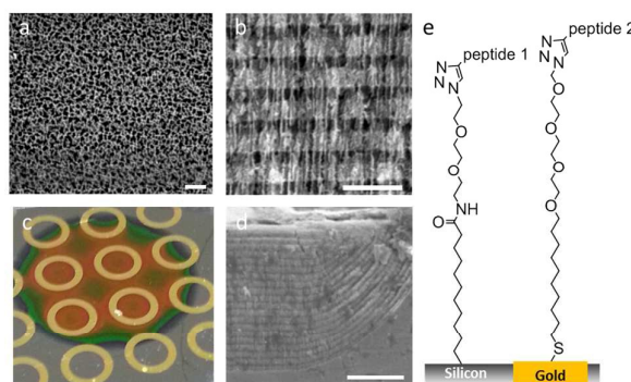
Figure 1. (a) Top view scanning electron micrograph of porous silicon. Scale bar 100 nm. (b) Side view scanning electron micrograph of Bragg mirror structure demonstrating alternating regions of low and high porosity. (c) Photograph of patterned gold rings on nanostructured porous silicon. (d) Side view scanning electron micrograph of porous silicon under-etched at the perimeter of a gold island. Scale bar 1 \mu m. (e) Schematic of functionalization chemistry for silicon and gold
