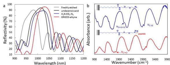
Figure 2. (a) Reflectivity spectra of a porous silicon Bragg mirror during chemical modification. (b) Fourier transform infrared characterization of chemical modification.
