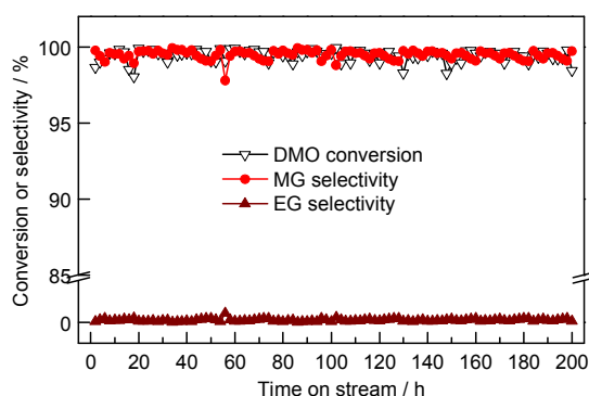
Fig. 6 Catalytic performance of Ag-in/hCNT as a function of reaction time. Reaction conditions: T = 493 K, P(\text{H}_2) = 3.0 MPa, \text{H}_2/\text{DMO} = 80 , \text{WLHSV} = 0.6 h -1 .
