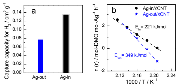
Fig. 2 Comparison of (a) \text{H}_2 chemisorption and (b) apparent activation energies. The symbol r means the reaction rate, moles of DMO converted by per mole of Ag per hour ( \text{mol-DMO mol-Ag}^{-1} \text{h}^{-1} ).
