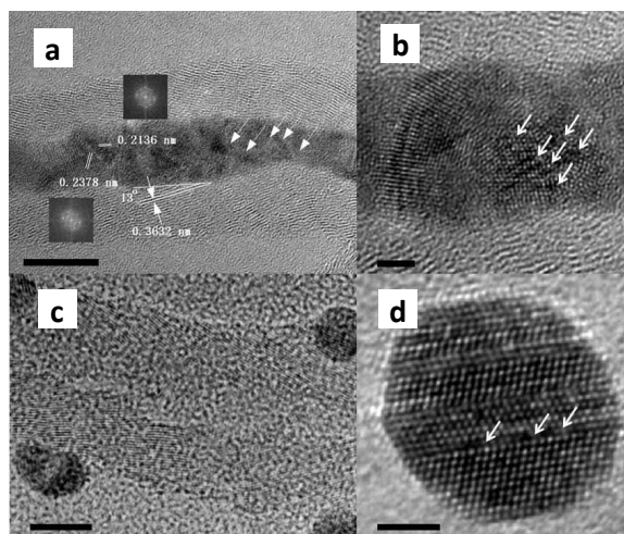
Fig. 3 High-resolution TEM images of (a) and (b) Ag-in/hCNT; (c) and (d) Ag-out/hCNT. The bar of (a) and (c) is 10 and 2 nm for (b) and (d). The inserted figures show the FFT change of Ag crystallites and were used to calculate lattice spacing. Arrows show the vacancies in Ag crystallites.
