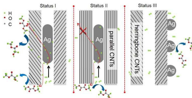
Scheme 1 Plausible scheme for the confinement and promotional effect of Ag/C hybrids.
