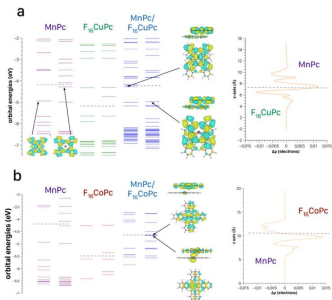
Figure 8. Electronic structure and charge density difference of the dimer model systems (a) MnPc/F_{16}CuPc and (b) MnPc/F_{16}CoPc .
