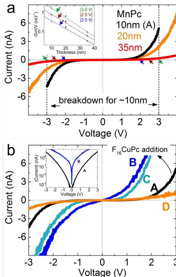
Figure 3. Current-voltage behavior for phthalocyanine-based heterojunctions, obtained via local AFM I-V spectroscopy. (a) Electrical characteristics for MnPc thin films with a thickness of 10 nm (sample A), 20 nm and 35 nm. Dashed lines indicate the threshold voltage where the thinner organic film (10 nm) suffers an electrical breakdown (see also supplementary information S3). The inset shows the conductance ( G ) of the films as a function of its thickness for \pm 3 V,
