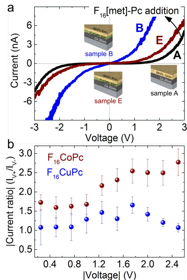
Figure 6. Transport dependence on the metallic center of the fluorinated phthalocyanine. (a) I-V transport characteristics of phthalocyanine heterojunctions, F_{16}CuPc/MnPc (sample B) versus F_{16}CoPc/MnPc (sample E). (b) Current rectification ratios ( |I_{v+}|/|I_{v-}| ) for the F_{16}CuPc and F_{16}CoPc systems considering both positive and negative voltages.
