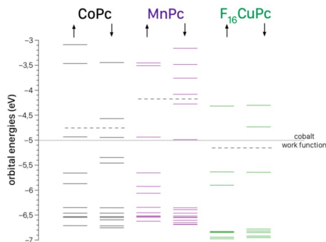
Figure 7. Ground state electronic structures of the metal phthalocyanine molecules as obtained from the DFT calculations. The dotted lines mark the Fermi levels of the individual molecules.
