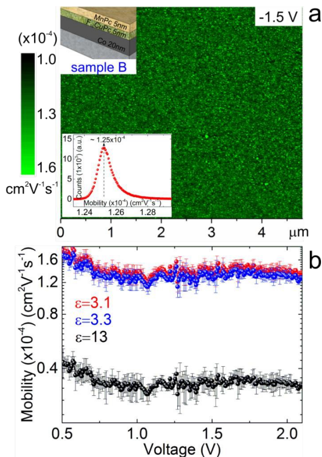
Figure 5. Nanoscale charge carrier mobility in F_{16}CuPc/MnPc heterojunctions. (a) Charge carrier mobility map obtained via dynamic cs-AFM at -1.5 V for the case of sample B. Inset shows the dispersion of charge mobility for the mobility map, considering an average of 512 \times 512 data points. (b) Mobility as a function of the applied voltage obtained via local I-V AFM spectroscopy, considering dielectric constants of 3.1, 3.3 and 13. The voltage range considered corresponds to the space-charge limited current transport regime identified in Figure 4. Error bars are obtained via standard deviation statistics taking into account data of about 40 local I-V cycles.
