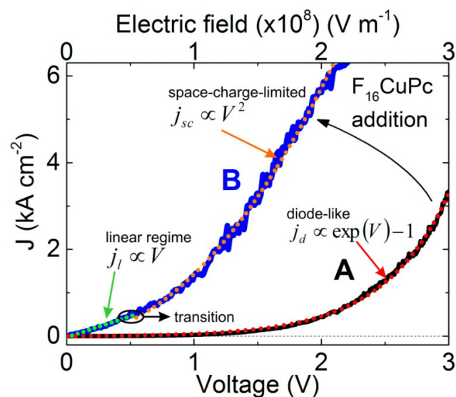
Figure 4. Transport mechanisms for metal phthalocyanine-based heterostructures. Solid lines represent the average of about 40 I-V cycles for sample A (black) and sample B (blue). Red dotted line corresponds to a diode-like transport regime for a 10 nm thick film of MnPc (sample A). Green and orange dotted lines show the transition from a linear to a space-charge-limited current (SCLC) transport mechanism for an F_{16}CuPc/MnPc heterojunction (sample B).
