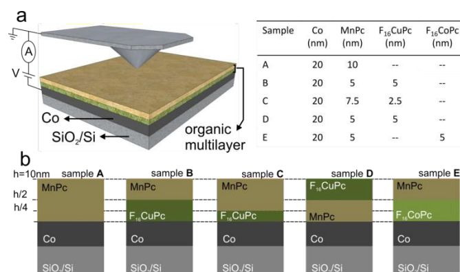
Figure 1. Experimental set up and organic heterostructure configurations. (a) Sketch of the cs-AFM set up for local transport measurements. (b) Phthalocyanine heterostructures: sample A (10 nm MnPc), sample B (5 nm F_{16}CuPc /5 nm MnPc), sample C (2.5 nm F_{16}CuPc /7.5 nm MnPc), sample D (5 nm MnPc/5 nm F_{16}CuPc ) and sample E (5 nm F_{16}CoPc /5 nm MnPc). All samples are deposited with a Co bottom electrode of 20 nm. The table provides the thicknesses for each layer in the samples.
