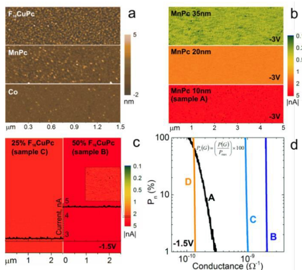
Figure 2. Topography and dynamic transport analysis of phthalocyanine organic heterojunctions. (a) AFM topography characteristics for Co substrate, MnPc and F_{16}CuPc thin films. (b) Thickness dependence of current maps for MnPc thin films obtained at -3 V. (c) Current maps for F_{16}CuPc/MnPc bilayer structures (samples B and C ) obtained at -1.5 V. Current map inset shows a zoom-in detail for an area of 1.5 \times 1.5 \mu m^2 with a higher current scale resolution. Current versus distance inset represents an average current profile for each sample. Due to the strong current dependence on the thickness of the organic material, all current maps are presented in a logarithmic scale. All current scales are presented in absolute value. (d) Electrical profile for the normalized distributions of conducting sites on organic films for samples A-D .
