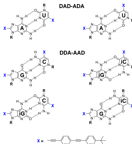
Figure 4. Triply H-bonded self-complementary base pair structures considered in this work.
