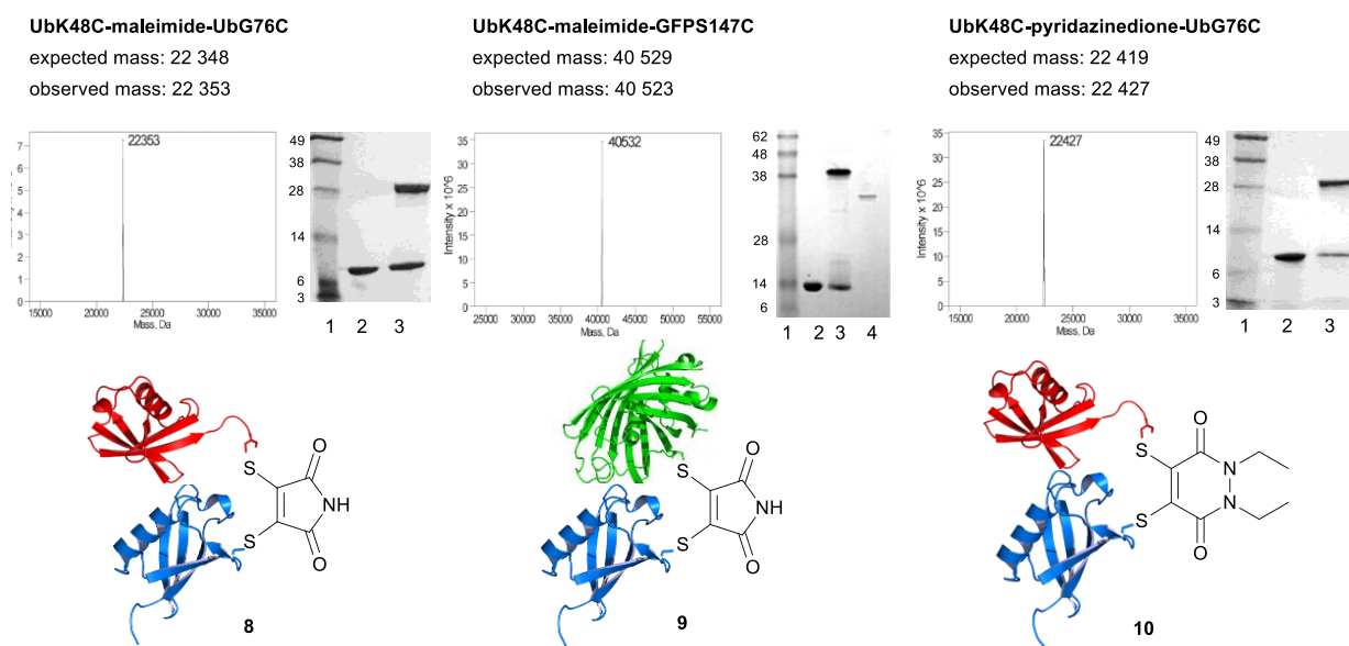
Fig. 3 Conjugation reactions for the formation of bis-protein conjugates 8-10 . Structures modified from PDB ID: 1UBQ and 2B3P. Lanes in SDS-PAGE gels are: 1-SeeBlue Plus2 ladder, 2-UbK48C, 3-coupling reaction, 4-GFPS147C. The band at ~11 kDa in lane 3 is due to excess ubiquitin.
