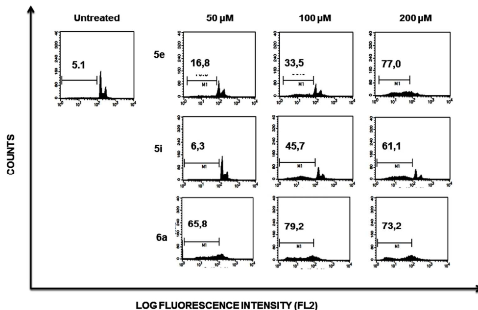
Effect of compounds 5e, 5i and 6a on cell cycle. A representative experiment showing Jurkat cells incubated for 48 h in the presence of indicated compounds and doses. Cell cycle subpopulations were analyzed by flow cytometry after permeabilisation and staining of cells with Propidium iodide. Additional controls containing equivalent amounts of DMSO used as drug vehicle were included, showing no toxicity in any case (not shown). Percentage of cells within the sub-G1 region are indicated in the plots. 254x190mm (96 x 96 DPI)
