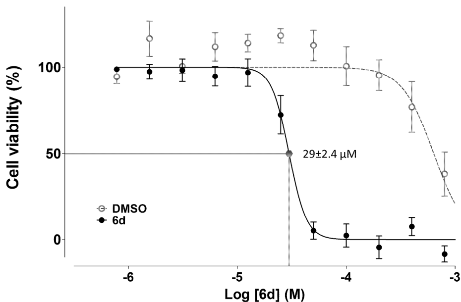
Figure 8.- IC 50 value of compound 6d in Jurkat cells as determined by inhibition of cell proliferation. A 11-point 1:2 serial dilution of compound 6d, starting at 800 μM, was used to determine its IC 50 value by the MTT assay after treatment of Jurkat cells for 48 h (solid circles). Equivalent amounts of DMSO used as vehicle in each dilution were set as negative controls (open circles). Results indicate percentages of cell proliferation over the results obtained with untreated cells. Data are expressed as mean ± SEM. 273x178mm (300 x 300 DPI)
