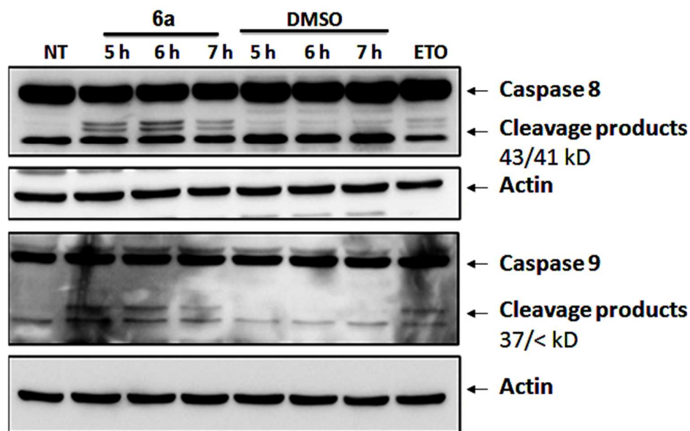
Figure 6. Study of early signaling events of apoptosis induced by compound 6a in Jurkat cells. Western blot analysis of total lysates of Jurkat cells after treatment with either compound 6a (200 \mu M, left-hand lanes) or equivalent amount of vehicle (DMSO, right-hand lanes) for 5, 6 or 7 h. Membranes were probed with antibodies against initiator caspases 8 or 9, using actin as loading control. Cells treated with Etoposide were included as positive control. Arrows indicate cleavage products (43/41 kD bands for caspase 8 and 37/< kD bands for caspase 9), which are detected after caspase activation whereas upper bands correspond to native proteins. Similar results were obtained after treating cells with compounds 5e and 5i (not shown). NT: Not
