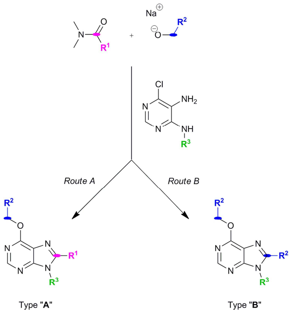
Scheme 1. Synthetic routes to generate purine types "A" or "B". Size of R1 controls which synthetic mechanism is followed under the same reaction conditions. 83x88mm (300 x 300 DPI)
