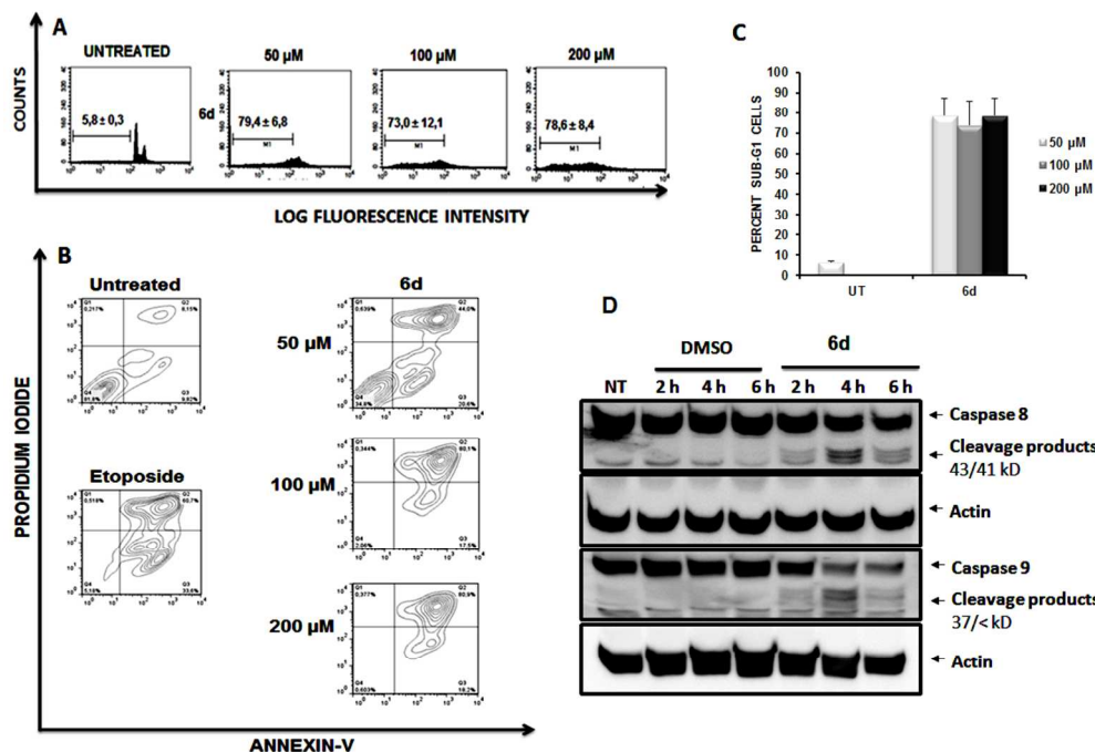
Figure 9. A) Effect of compound 6d on the cell cycle of Jurkat cells. Jurkat cells were treated for 48 h with 6d at indicated concentrations or their equivalent amounts of DMSO used as vehicle. Cells gated on the sub-G1 region after staining with propidium iodide are indicated. B) Membrane phosphatidylserine expression after treatment of Jurkat cells with compound 6d. Jurkat cells were treated for 24 h with compound 6d and the indicated doses and the percentages of apoptotic cells was measured by flow cytometry after double staining with propidium iodide and Annexin-V-Fluos. Dot plots represent the results of a typical experiment. Untreated cells and cells exposed to Etoposide were included as negative and positive controls. C) Percentages of apoptotic cells after treatment of Jurkat cells with compound 6d. Graph summarizes values of percentages of apoptotic cells and SEM obtained from three independent experiments. UT: Untreated. D) Activation of initiator caspases 8 and 9 after cell treatment with compound 6d. Western blot analysis of total lysates from Jurkat cells after treatment with either compound 6d (200 μM, right-hand lanes) or vehicle (DMSO, left-hand lanes) for 2, 4 and 6 h. Membranes were probed with antibodies against initiator caspases 8 or 9, using actin as loading control. Arrows indicate cleavage products (43/41 kD bands for caspase 8 products and 37/< kD bands for caspase 9 ones) after caspase activation whereas upper bands correspond to native proteins (caspase 8 correspond to 55/57 kD band and caspase 9 to 45 kD band)
