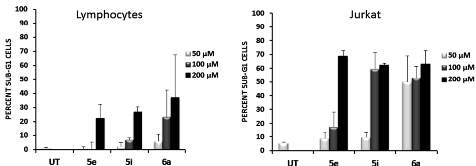
Figure 5. Effect of indicated compounds on primary lymphocytes and Jurkat cells. Primary cell line N1 and Jurkat cells were treated for 48h at the indicated doses of compounds 5e, 5i and 6a and cell cycles were analysed by flow cytometry after staining with Propidium Iodide. Graphs represent the mean \pm S.D. of cells gated within the sub-G1 region obtained from three independent experiments. UT: Untreated. 254x108mm (96 x 96 DPI)
