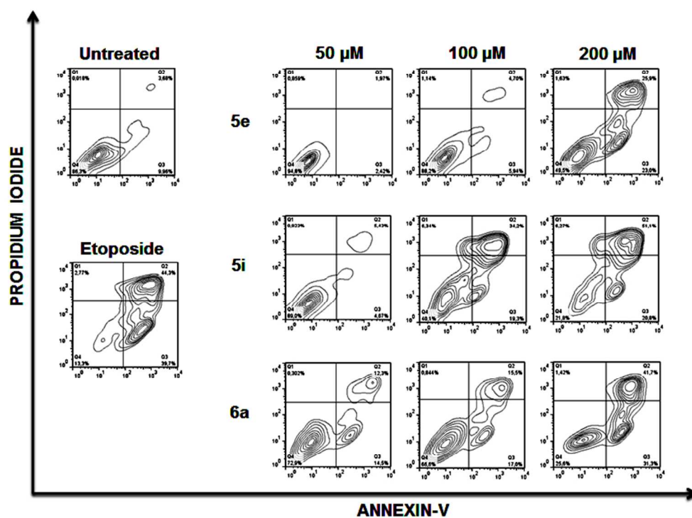
Figure 4. Membrane phosphatidylserine expression after treatment of Jurkat cells with compounds 5e, 5i and 6a. Jurkat cells were treated for 48 h with the indicated compounds and doses and the percentages of apoptotic cells was measured by flow cytometry after double staining with propidium iodide and Annexin-V-Fluos. Dot plots represent the results of a typical experiment. Untreated cells and cells exposed to Etoposide were included as negative and positive controls.
