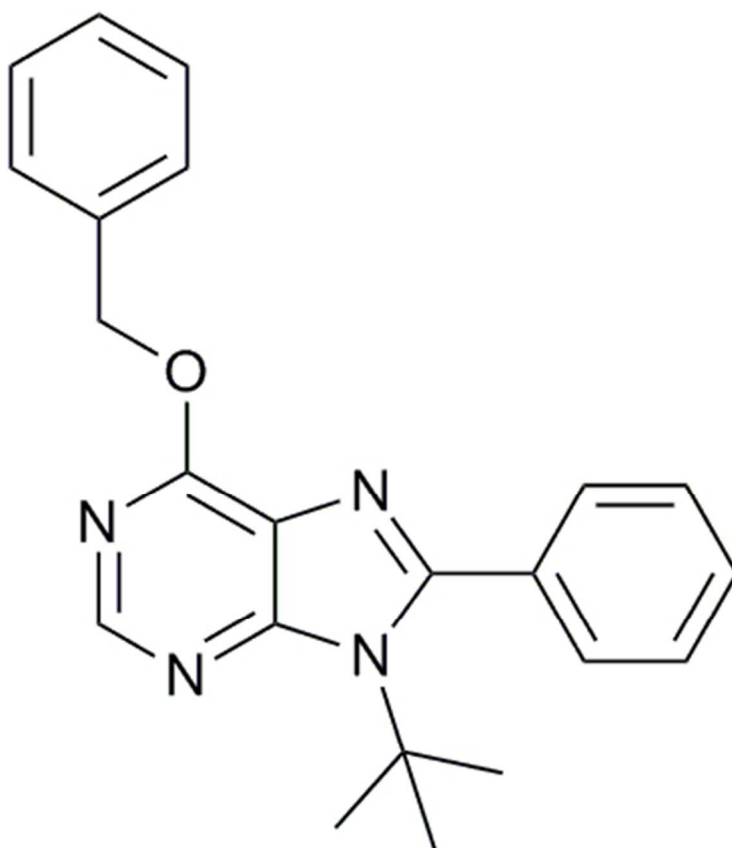
Figure 7. Structure of compound 6-benzyloxy-9-tert-butyl-8-phenyl-9H-purine 6d. 32x36mm (300 x 300 DPI)
