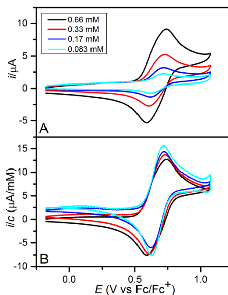
Fig. 5. The influence of the substrate concentration (see the insert) on the shape of the cyclic voltammogram for \mathbf{2}_{\text{PhePhe}} . (A) the raw data and (B) the same data after background subtraction and normalization with respect to the substrate concentration. The working electrode was a circular glassy carbon disk ( d = 3 mm); the voltage sweep rate was 0.1 \text{ Vs}^{-1} .
