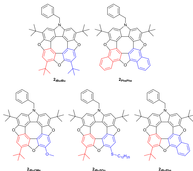
Fig. 1. Azatrioxa[8]circulenes ( 2 ) described in this paper.
