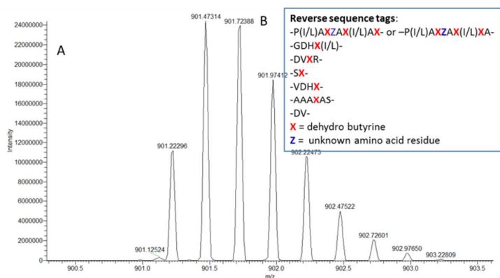
Figure 2. (A). Mass spectrometric identification of the 3600 Da legonaridin 1 from the organic extract of Streptomyces sp. CT34 (ion [M+4H]^{4+} ); (B) Generation of 7 reverse sequence tags from the purified legonaridin 1 by FTICR-mass spectrometric detection. X = dehydrobutyryne and Z = unidentified amino acid residue.
