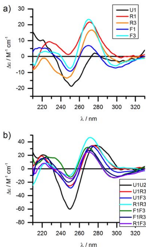
Fig. 2. CD spectra of the DNA region of LNA-porphyrin modified ODNs (selected representative examples) in a) single stranded and b) double stranded form. 4 \mu\text{M} DNA, 50 mM phosphate buffer, 100 mM NaCl, 1 mM \text{Na}_2\text{EDTA} , pH 7.0.
