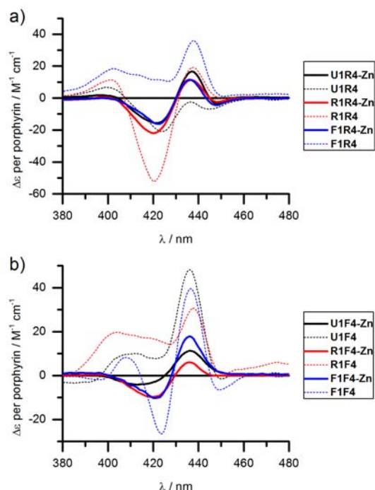
Fig. 4. CD spectra of zinc metallated porphyrin arrays, containing either a) R4-Zn or b) F4-Zn, in comparison with the non-metallated duplexes. \Delta\epsilon values are given per porphyrin (normalized to the number of porphyrins present). Conditions as in Fig. 2.
