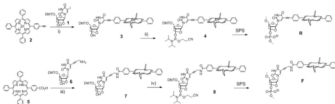
Scheme 1. Synthesis of the building blocks and DNA sequences. Reagents and conditions: i) Pd(PPh 3 ) 4 , CuI, TEA, DMF, 91%; ii) CEP-Cl, DIPEA, DCM, quant.; iii) EDC, HOBt, DMAP, DCM, 68%; iv) CEP-Cl, DIPEA, DCM, quant. SPS: Solid Phase Synthesis of DNA.
