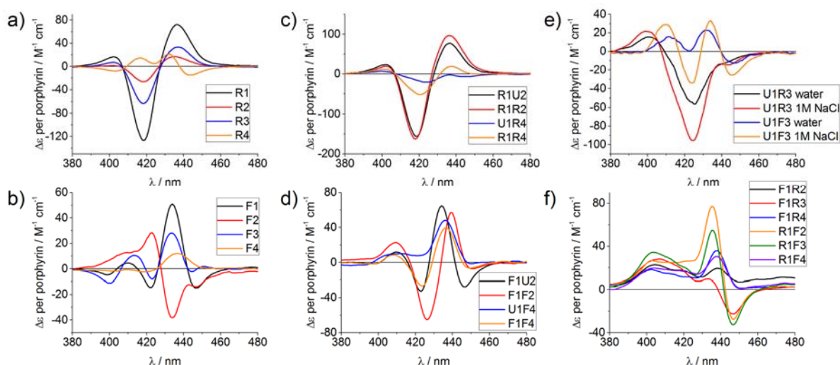
Fig. 3. CD spectra of porphyrin-LNA strands of selected examples showing the porphyrin region of the spectra. a) and b) spectra of single strands with LNA-1 or LNA-2 modification, respectively. c) and d) spectra for selected duplexes where the same modifier has been used in both strands. e) Comparison of stands U1•R3/F3 in pure water or in 1 M NaCl (50 mM phosphate buffer) solution. f) Mixed LNA duplexes where the complementary strands have been modified with different modifiers. \Delta\epsilon values are given per porphyrin (normalized to the number of porphyrins present). Conditions as in Fig. 2.
