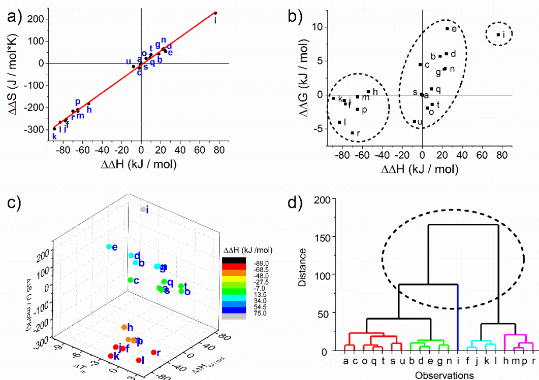
Figure 1. Thermodynamic plots of the porphyrin-LNA duplexes. Data are taken from Table 1. a) enthalpy-entropy compensation with linear regression [ \Delta\Delta S = -5.88 + (3.15 \text{ K})\Delta\Delta H ; R^2 = 0.996 ]. b) Correlation between \Delta\Delta H and \Delta\Delta G^{298} demonstrating that there is a linear correlation between \Delta\Delta G and \Delta\Delta H . 66 c) enthalpy-entropy-change in \Delta T_m correlation showing further clustering when compared to net change of entropy. d) Hierarchical analysis using the euclidean distance carried out by OriginLab software presenting five clusters of duplex samples. The dashed circle indicates the classification of the three groups identified in a), b) and c); the main groups can be further divided into five major subgroups.
