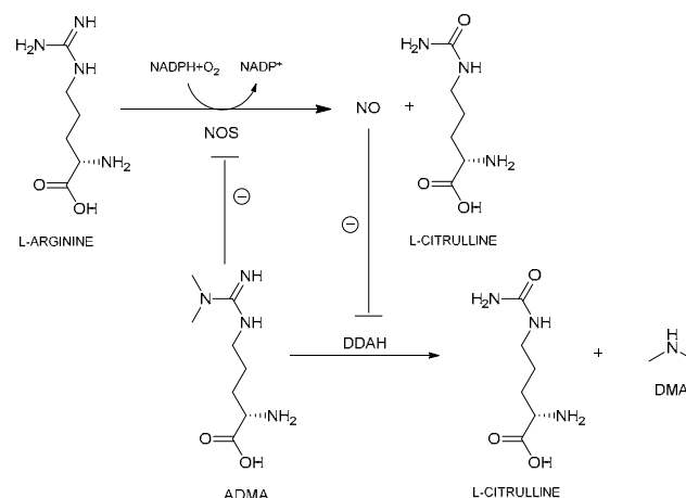
Figure 1. Schematic diagram highlighting the overlap between DDAH and NOS biochemical pathways.
