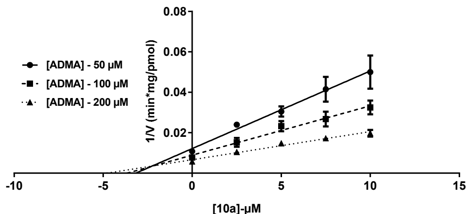
Figure 3. Dixon plot of 10a inhibition of L-citrulline formation by DDAH-1: experimentally determined values (points), model fitted curves of the best fit (lines).
