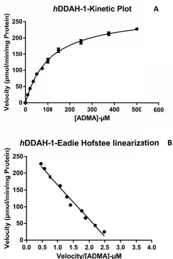
Figure 6. (A) Rate of reaction (pmol/min/mg protein) versus [ADMA] plot of L-citrulline formation by hDDAH-1. (B) Eadie-Hofstee plot for L-citrulline formation induced by hDDAH-1 at different ADMA concentrations. Units of Velocity/[ADMA] are pmol citrulline/ \mu\text{mol} / min / mg. Points are experimentally determined values, whereas lines are from model-fitting.
