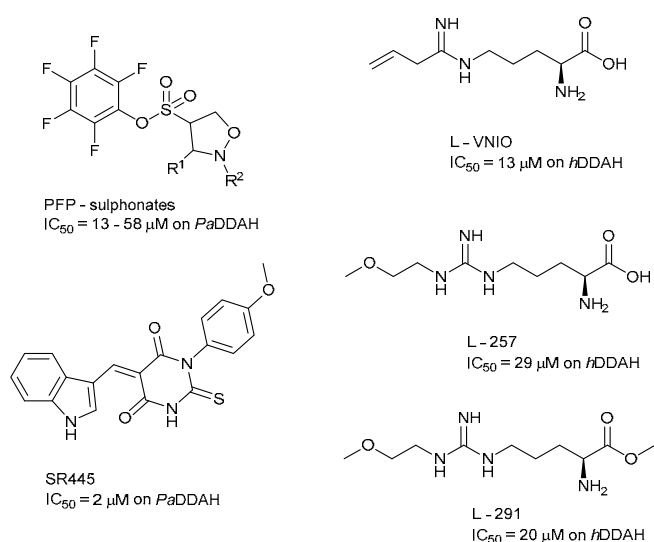
Figure 2. 22,32 Current DDAH inhibitors reported in the literature with their IC 50 values.
