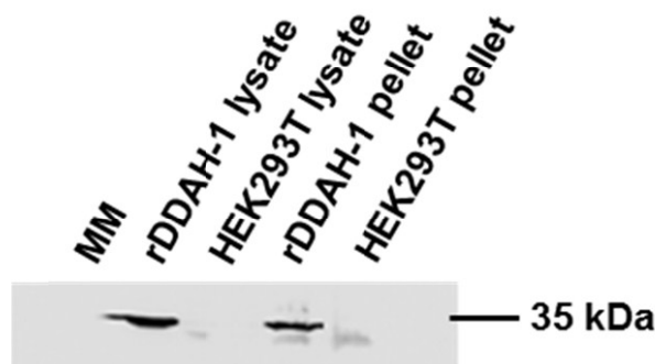
Figure 5. Immunoblot of human DDAH-1 expression. HEK293T cell lysate (50 \mu\text{g} ) and pellet (50 \mu\text{g} ) were resolved by SDS-PAGE, blotted to nitrocellulose, and probed with anti-DDAH-1 antibody. Molecular weight markers (MM; lane 1), recombinant DDAH-1 lysate (lane 2), untransfected HEK293T control cell lysate (lane 3), recombinant DDAH-1 pellet (lane 4), untransfected HEK293T control cell pellet (lane 5). The immuno-reactive bands occur at 35 kDa.
