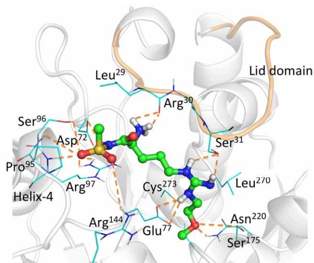
Figure 4. The favoured binding mode of molecule 10a (ball and stick) observed in molecular dynamics simulations (average configuration from 50ns time scale). Green = carbon; red = oxygen; blue = nitrogen; yellow = sulphur. Only hydrogen atoms (white) involved in hydrogen bonds are shown for clarity. Hydrogen bonds are shown in dashed orange lines, with the 'lid' domain shown as a beige loop (residues 29-39). Secondary structure of DDAH-1 is rendered (cartoon).
