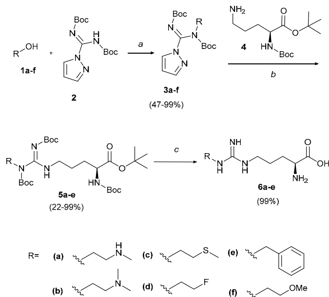
Scheme 1. L-257 side-chain derivatives synthesis. Reaction conditions: a. Ph 3 P, DIAD, THF, 0°C-rt, 16 h, 47-99%; b. DIPEA, DCM, rt, 24 h, 22-99%; c. TFA, DCM, rt, 3 h, 99%.
