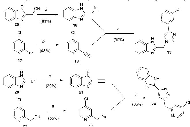
Scheme 4. Triazoles synthesis. a. DPPA, DBU, toluene, rt, 16 h, 55-85%; b. (Ph 3 P) 2 PdCl 2 , CuI, TEA, ethynylTMS, 80 °C, 20 h, 48%; c. CuI, sodium ascorbate, TEA, DCM, rt, 24 h, 30-65%; d. (Ph 3 P) 2 PdCl 2 , CuI, TEA, TIPS-acetylene, DMF, 80 °C, 72 h, 30%.
