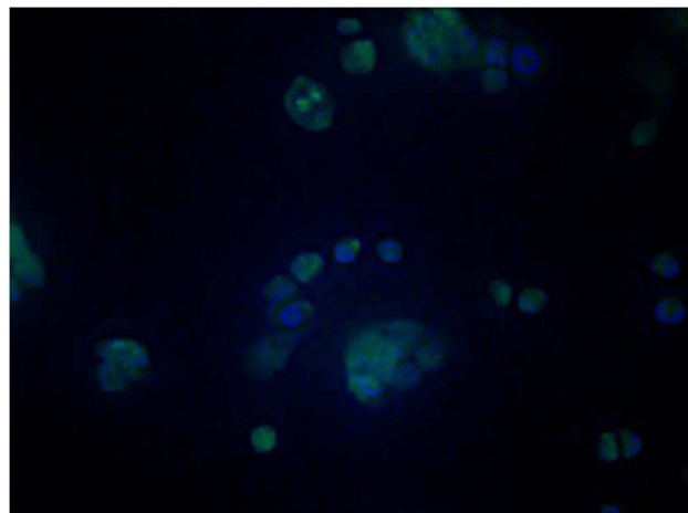
Figure 4. Showing co-localisation DAPI and drug in the nucleus of A549 cells. Magnification: 40x, green: 11-chloro cryptolepine, blue: DAPI nuclear dye, Overlay of both drug and DAPI
