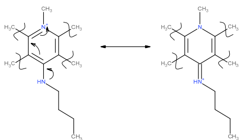
Figure 1. Possible resonance structure for 11-aminocryptolepine derivatives.
