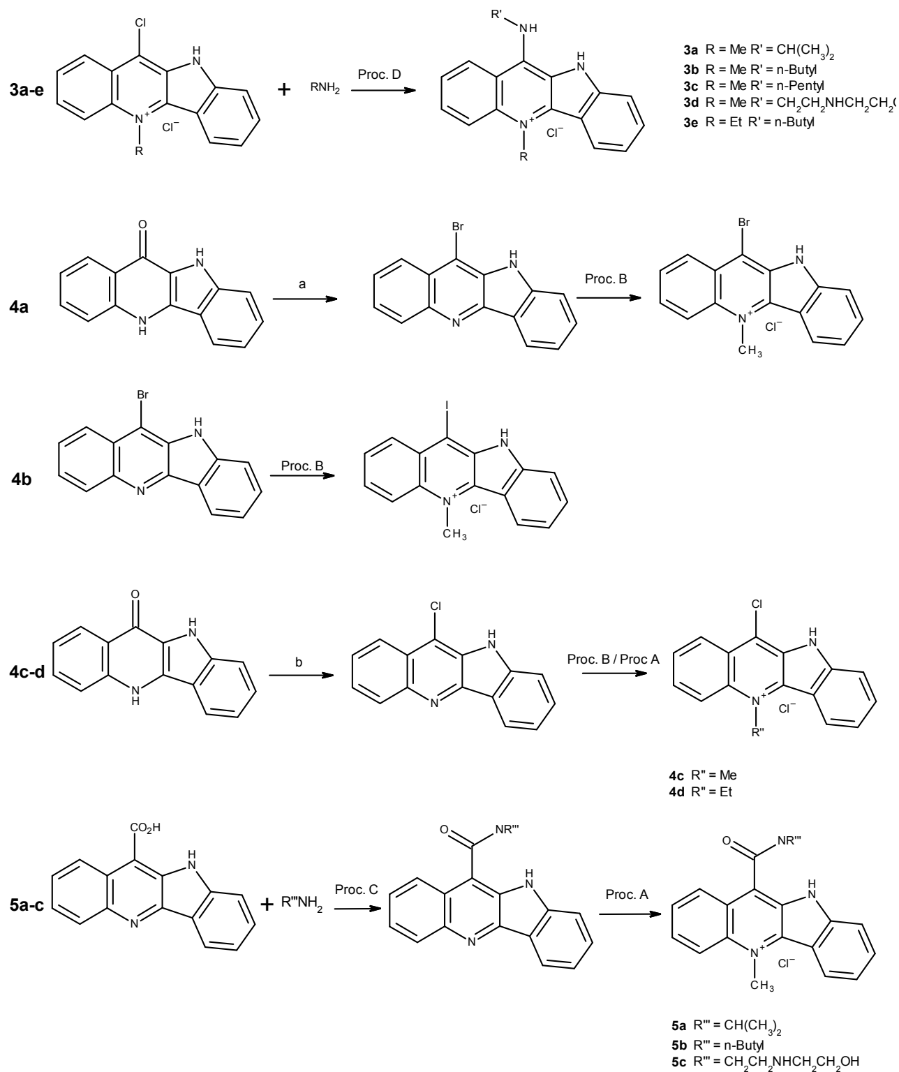
Scheme 1. Synthetic route for the cryptolepine derivatives. (a) POBr 3 , PBr 3 , 16hrs, reflux (b) POCl 3 , PCl 5 , 4 hrs reflux. General procedures are given as Proc. A-D and are discussed in more depth in the methods section: (A) methyl/ethyl triflate, 34hrs, RT (B) MeI, Sulfolane 16hrs RT (C) COMU, Et 3 N, DCM 16hrs RT (D) EtOAc, amine, 16 hrs, reflux.
