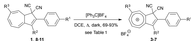
Scheme 3. Synthesis of azulonium tetrafluoroborate salts 3-7 . DCE = 1,2-dichloroethane.
