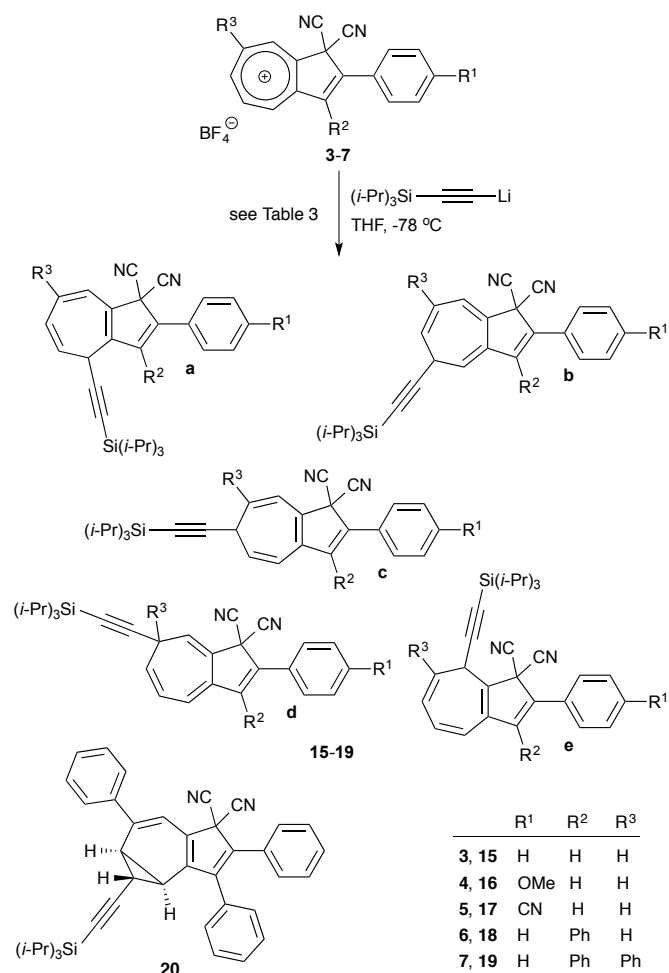
Scheme 4. Addition of triisopropylsilylacetylide anion to azulonium ions 3-7 .
