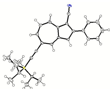
Figure 4. Top: Molecular structure of 23 (CCDC 1441531). The crystals were grown from evaporating ethyl acetate. The blue sphere represents nitrogen and the yellow sphere silicon.
