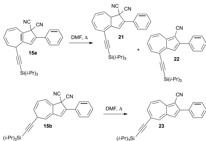
Scheme 5. Tautomerization of dihydroazulene products.
