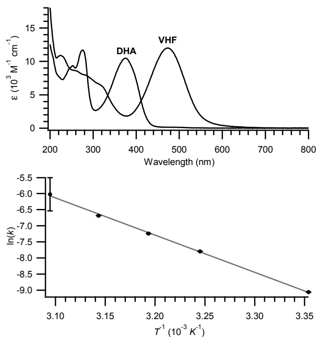
Figure 5. Top: Absorption spectra of DHA 21 and its corresponding VHF 24 in MeCN at 25 °C. Bottom: Arrhenius plot for the thermal VHF to DHA ring-closure. E_a = 95.8 \pm 1.9 \text{ kJ/mol} and A = 7.10 \times 10^{12} \text{ s}^{-1} .
