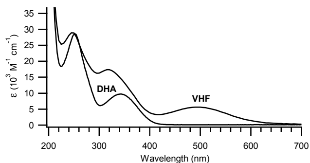
Figure 3. UV-Vis absorption spectra of pure DHA 11 and the corresponding VHF in MeCN at 25 °C. On account of the fast VHF to DHA conversion, the spectrum of VHF contains overlapping DHA absorptions.
