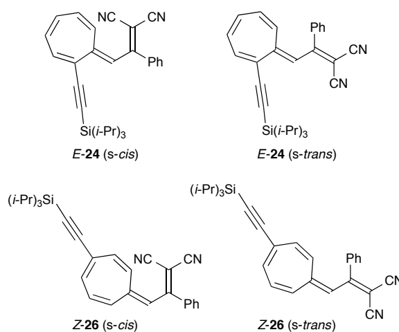
Figure 6. Conformations of VHF E-24 and Z-26 .
