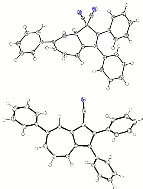
Figure 2. Top: Molecular structure of 11 (CCDC 1441529). The crystals were grown from dichloromethane/ethanol. Bottom: Molecular structure of 14 (CCDC 1441530). The crystals were grown from THF/heptane. The blue spheres represent nitrogen atoms.
