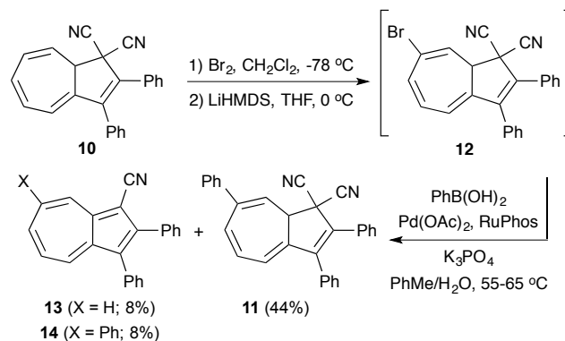
Scheme 2. Synthesis of 2,3,7-triphenyl-substituted DHA 11 . RuPhos = 2-dicyclohexylphosphino-2',6'-diisopropoxybiphenyl.
