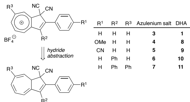
Figure 1. Retrosynthetic route to azulonium salts 3-7 by hydride abstraction from DHA precursors 1, 8-11 .
