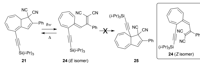
Scheme 6. Ring-opening/closure of DHA 21 .
