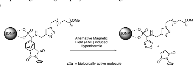
Scheme 1 The concept of magnetically stimulated rDA reaction using IONPs
