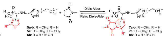
Scheme 3 DA and rDA reactions between furan-functionalized PEO monomethyl ethers and N -methylmaleimide
