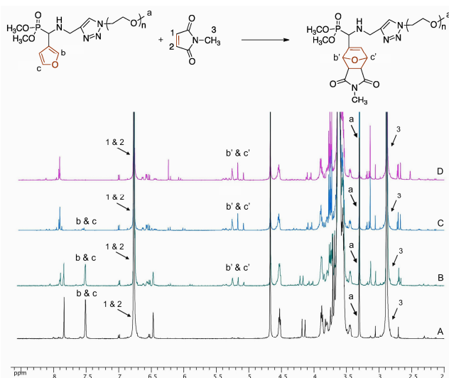
Fig. 1 Overlay of 1 H NMR spectra of the reaction mixture of 5b and N -methylmaleimide for a [N\text{-methylmaleimide}]/[5b] molar ratio of 20 in D 2 O at 40°C recorded for a reaction time of (A) t = 0 , (B) t = 3 h, (C) t = 1 day and (D) t = 3 days
