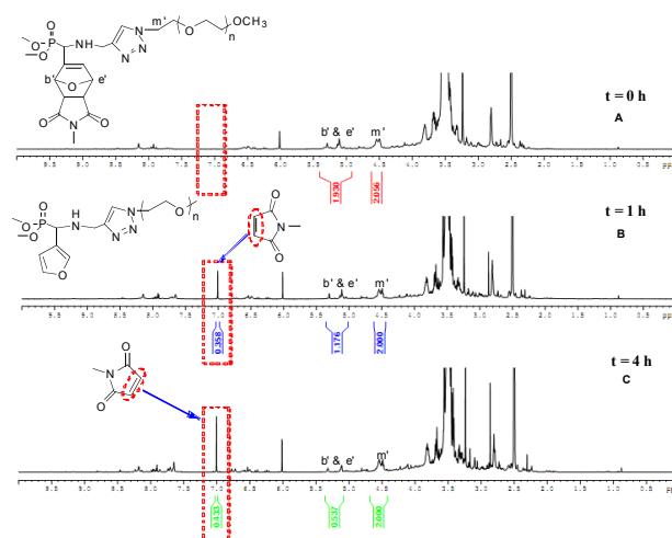
Fig. 4 1 H NMR spectra of the rDA reaction of 7b in DMSO-d 6 at 110 °C for (A) t = 0 h, (B) t = 1 h et (C) t = 4 h
