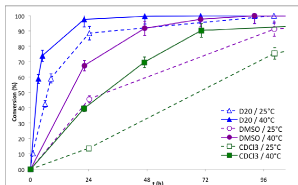
Fig. 2 Conversion of the DA reaction between 5b and N -methylmaleimide in different solvents at 25°C and 40°C versus time
