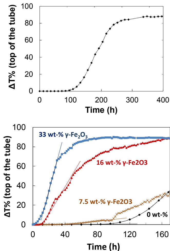
Figure 9. Relative transmission intensity \Delta T (in %) at the top of the tube ( H = 35.6 \text{ mm} \pm 1.0 ) as a function of time for OEGDA-crosslinked P(MEO 2 MA-co-OEGMA-co-MAA) microgels (top, 0 wt-% of NP, \blacklozenge ) and for \gamma\text{-Fe}_2\text{O}_3 -P(MEO 2 MA-co-OEGMA-co-MAA) hybrid microgels (bottom, 0 ( \blacklozenge ), 7.5 ( \times ), 16 ( \blacktriangle ), 33 ( \blacksquare ) wt-% of NP) as a function of time (solid content \tau = 2.1 \text{ wt-}\% ).
