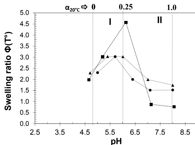
Figure 6. Temperature-induced swelling ratio ( \Phi_{T^0} ) as a function of pH for P(MEO 2 MA- co -OEGMA- co -MAA) microgels crosslinked with OEGDA (▲), MBA (●) or EGDMA (■).
