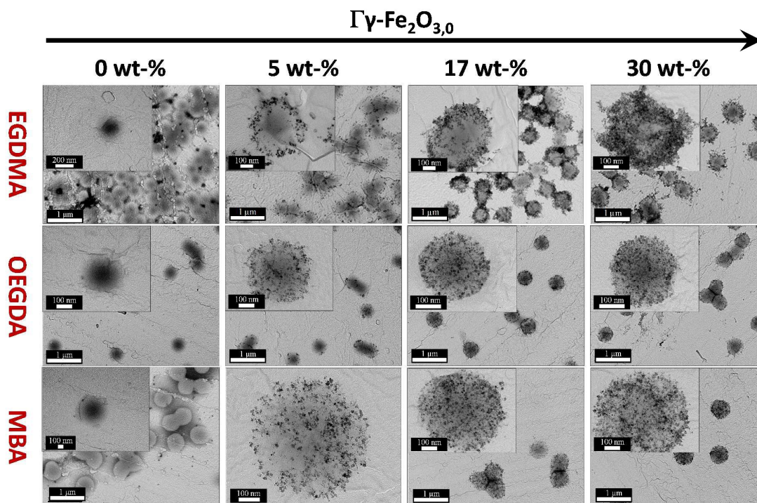
Figure 8. Transmission electron micrographs of P(MEO 2 MA- co -OEGMA- co -MAA) microgels and \gamma -Fe 2 O 3 -P(MEO 2 MA- co -OEGMA- co -MAA) hybrid microgels crosslinked with EGDMA, OEGDA or MBA. \Gamma_{\text{Fe}_2\text{O}_3,0} is the initial weight content of NPs added into the microgel dispersion relative to the polymer weight.
