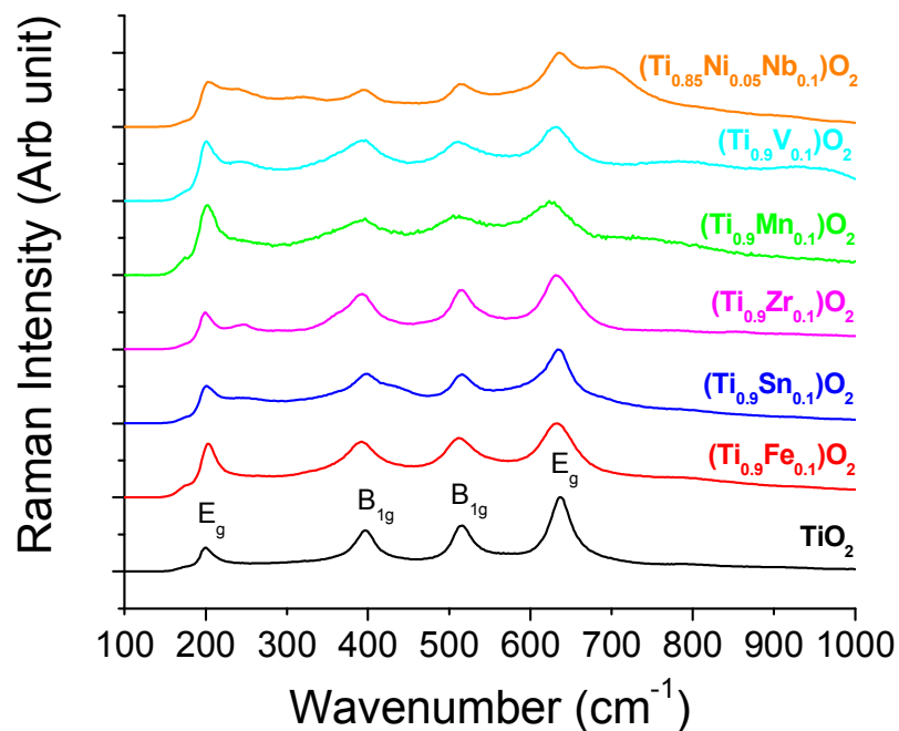
Figure 4 Raman spectra of transition-metal containing \text{TiO}_2 . Pure \text{TiO}_2 shows Raman bands at 200, 396, 515, and 637 \text{cm}^{-1} .
