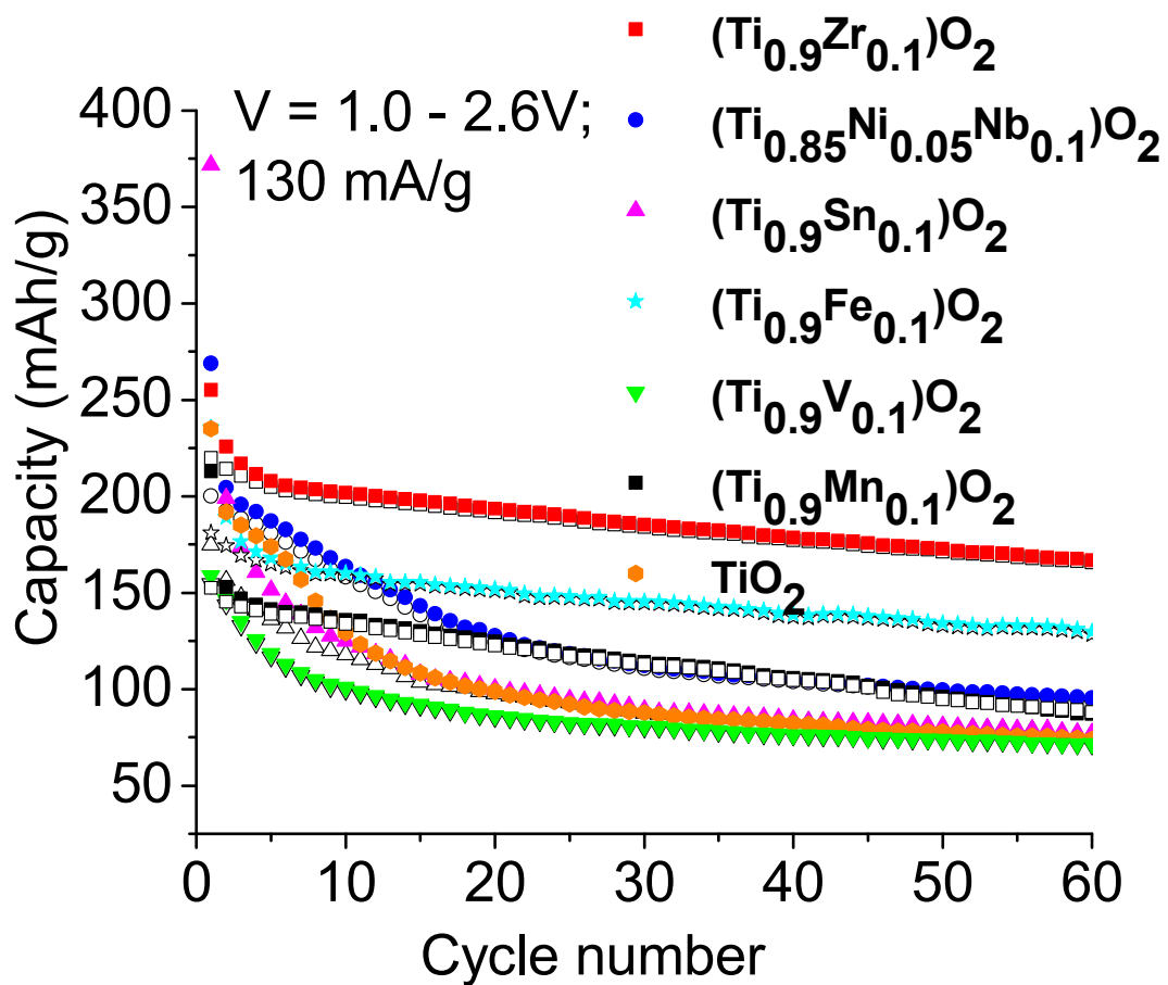
Figure 7. Capacity vs. cycle plots of pure and doped TiO 2 from 1 st to at least 60 cycles in the voltage range 1.0 – 2.6 V vs. Li with a current density of 130 mA g -1 . Filled and open symbols represent discharge and charge capacities, respectively.
