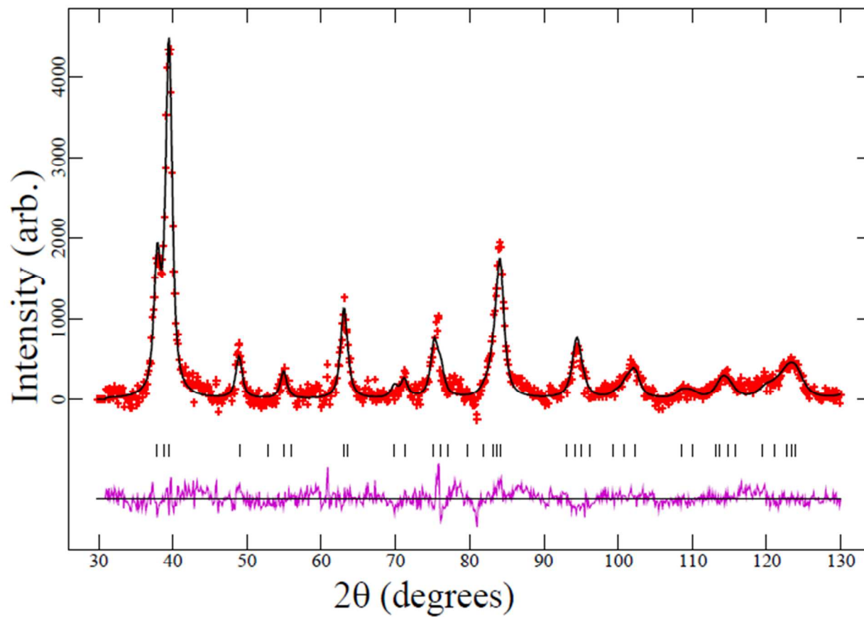
Figure 2. Rietveld-refinement profile using the anatase \text{Ti}_{0.9}\text{Mn}_{0.1}\text{O}_2 NPD data. The red crosses are the data, the black line through the crosses is the calculated Rietveld model, the purple line below is the difference between the data and calculated model, and the vertical black-lines are reflection markers for anatase.
