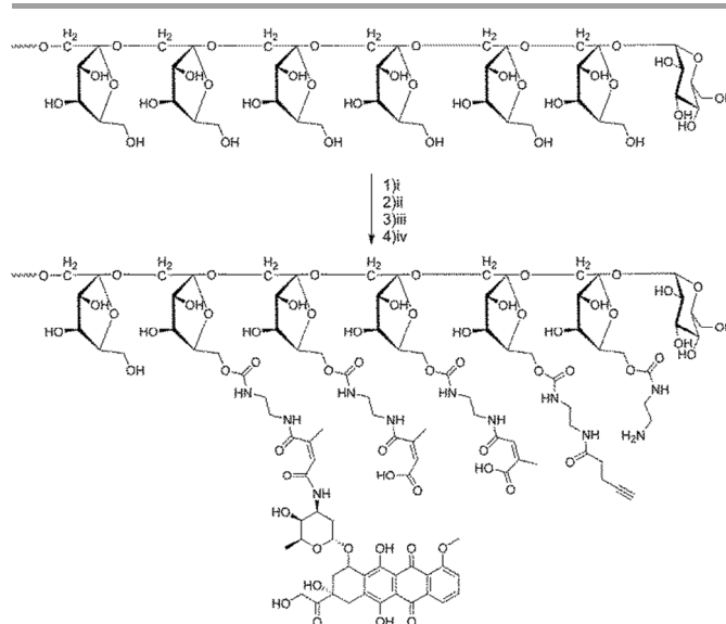
Scheme 1. Synthesis of INU-EDA-P,C-Doxo: i) Bis(4-nitrophenyl) carbonate, 4h, 40°C, 40'; EDA; ii) EDC HCl, NHS, pentynoic acid, pH 6.8, r.t., 18h; iii) Citraconic anhydride, NaOH, pH 8-9, 2h; iv) EDC HCl, NHS, doxorubicin hydrochloride, pH 6.8, r.t., 18h
