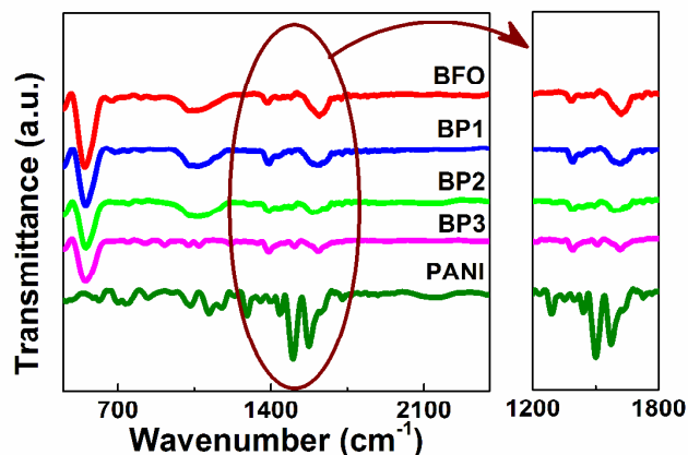
Fig. 3 FTIR spectra of BFO, BP1, BP2 and BP3 samples.
