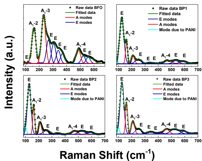
Fig. 4 Raman Spectra for BFO, BP1, BP2 and BP3 samples.
