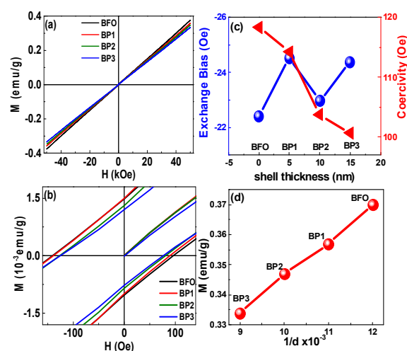
Fig. 5 Room Temperature hysteresis loops for BFO, BP1, BP2, BP3 (a), expanded view of the hysteresis loops (b), Plot of exchange bias and coercivity as a function of shell thickness (c) and plot of 1/d and magnetization as a function of shell thickness (d).
