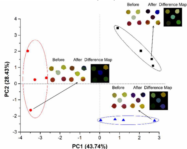
Fig. 4 PCA scores plot obtained from the RGB values extracted from the coloured membranes with 5 pH indicators in contact with volatile phase collected from a chamber containing meat contaminated with: ■ – isobutylamine; ● – triethylamine and ▲ – isopentylamine. Highlighted images show the real images of the colour changes profile of the sensor array for one of the experiments before and after the exposition of meat contaminated with each amine and respectively difference map for each experiment.
