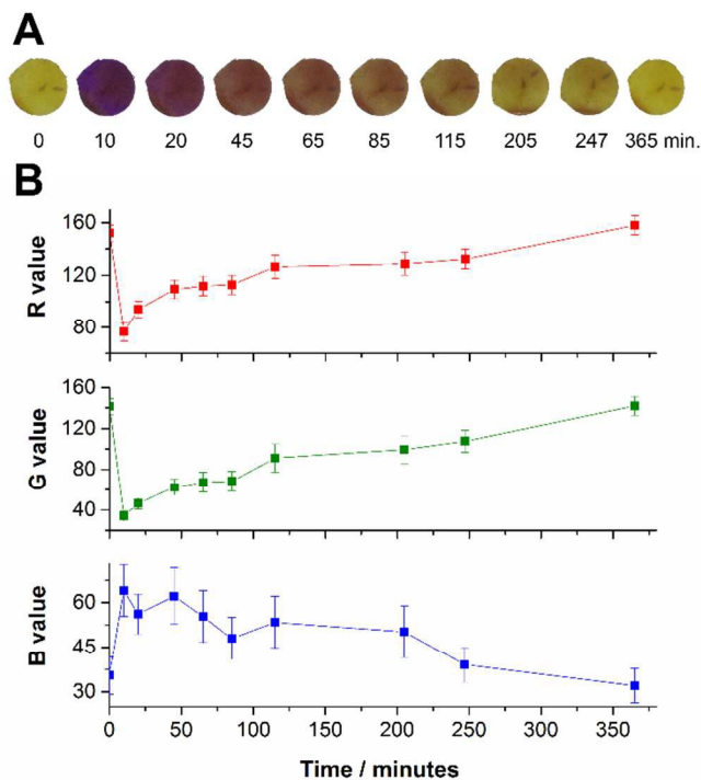
Fig. 3 Regeneration test monitoring: images obtained for each experiment time (A) and the R, G and B values for the spot number 3 Fig. 1 (chlorophenol red) (B). Number of replicates = 3.
