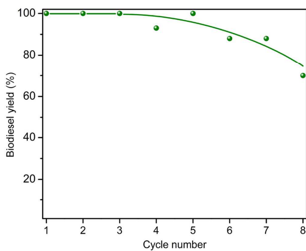
Figure 6. Soybean oil-to-biodiesel conversion yield (%) versus number of catalytic cycles for the CaGEO-4 catalyst under the same refluxing condition at 67 °C. After each cycle, the catalyst was washed and calcined.
