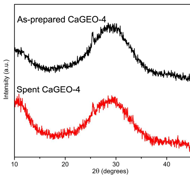
Figure 7. Powder X-ray diffraction patterns of as-prepared and spent catalyst CaGEO-4.
