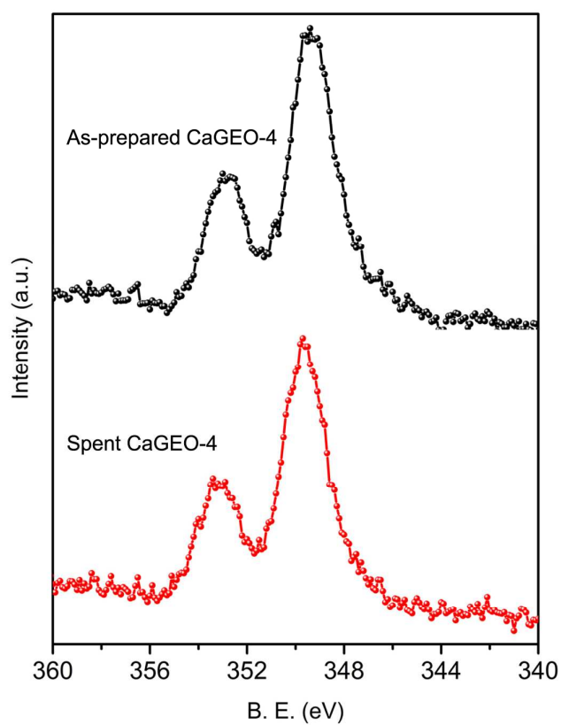
Figure 2. Ca(2p) core level spectra of as-prepared and spent catalyst CaGEO-4. Binding energies are corrected using C(1s) at 284.5 eV.
