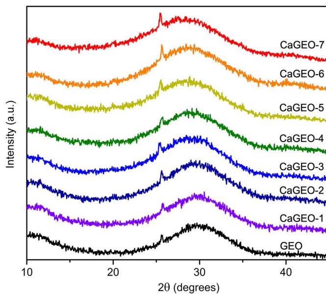
Figure 1. Powder X-ray diffraction patterns of unmodified geopolymer (GEO) and calcium-modified geopolymers (CaGEO-1 to -7) from bottom to top. See Table 1 for the details of the samples. The small sharp peak at 25.3° is from an anatase TiO 2 impurity (PDF# 00-021-1272) in the metakaolin.
