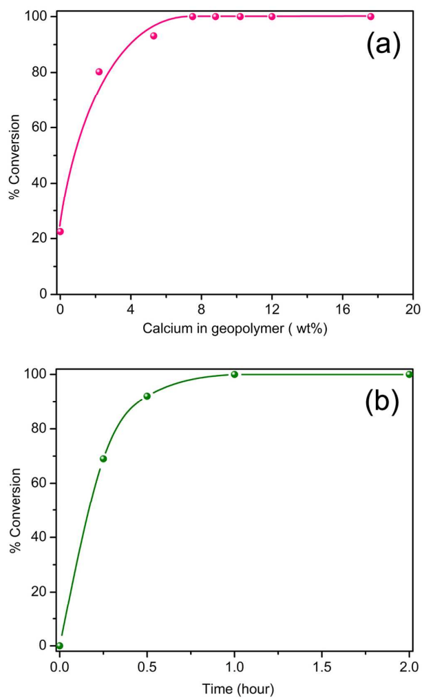
Figure 5. Soybean oil-to-biodiesel conversion yield (%) for calcium modified geopolymer catalyst as a function of calcium amount (a), and as a function of reaction time (b) under the same refluxing condition at 67 °C for CaGEO-4.
