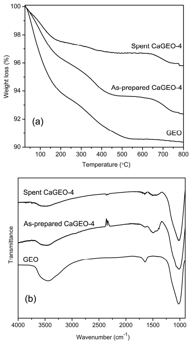
Figure 8. TGA thermograms (a) and FT-IR spectra (b) of GEO, as-prepared CaGEO-4, and spent CaGEO-4 after 8 catalytic cycles.
