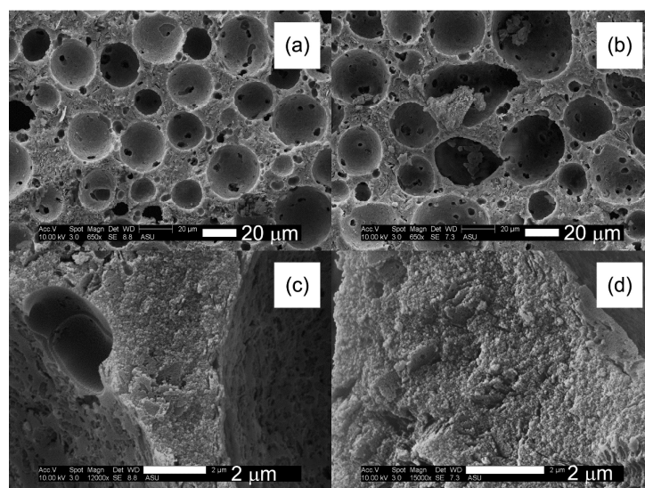
Figure 4 SEM images of GEO in (a) and (c) (scale bar = 20 and 2 μm, respectively) and of CaGEO-4 in (b) and (d) (scale bar = 20 and 2 μm, respectively).
