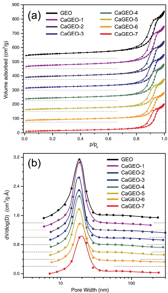
Figure 3. N_2 gas isotherms (a), and BJH pore distribution curves (b) of unmodified geopolymer (GEO) and calcium-modified geopolymers (CaGEO-1 to -7) from top to bottom. The grey dashed lines indicate the zero starting points for the vertical axis. See Table 1 for the details of the samples.
