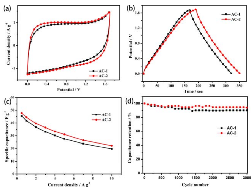
Fig. 7 Electrochemical performances for both of symmetric supercapacitor in \text{NaNO}_3
