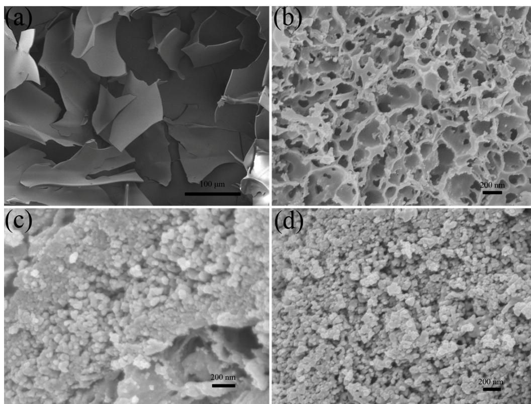
Fig. 2 SEM image of the porous carbon materials: SL based biochar (a); AC-1 (b); SL based biochar after carbonization (c); AC-2 (d).
