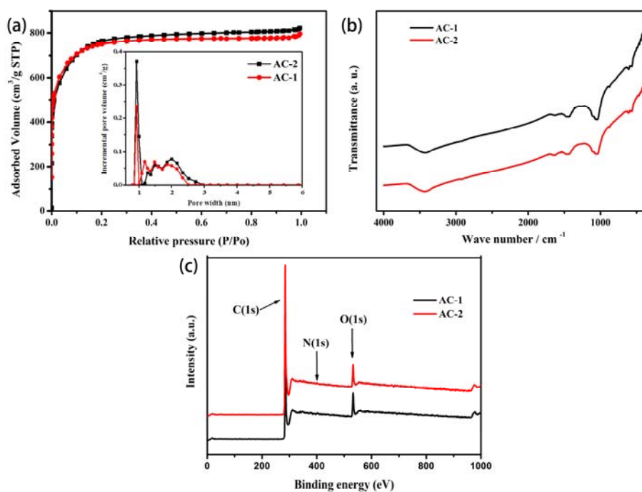
Fig. 3 (a) Nitrogen adsorption isothermal curves of AC-1 and AC-2 samples, the inset is the pore size distributions of the corresponding materials, which are calculated by
