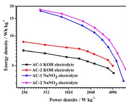
Fig. 8 Ragone plot for the symmetrical capacitors based on AC-1 and AC-2 in KOH and \text{NaNO}_3 electrolyte, respectively.
