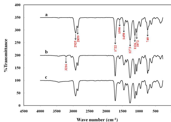
Figure 6: Comparison of FT-IR spectra for membrane ingredients under different conditions: (a) blank membrane without p-IPC6 as ionophore, (b) fabricated membrane with ionophore and (c) used membrane after 3 months.
