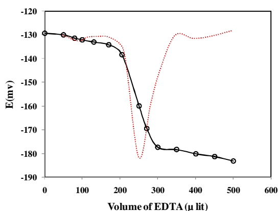
Figure 9: Potentiometric titration curve of cesium ion ( 1.0 \times 10^{-4} M, 25 mL) with standard EDTA solution ( 1.0 \times 10^{-2} M) using fabricated electrode based on p-IPC6 as an indicator electrode.
