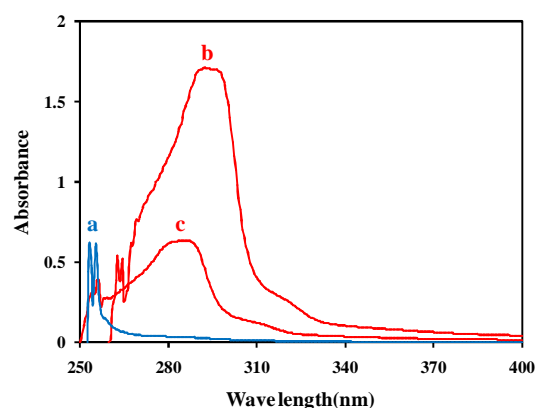
Figure 7: UV-Vis absorption spectra: (a) 1.0 \times 10^{-3}\text{ M Cs}^+ , (b) 1.0 \times 10^{-4}\text{ M p-IPC6} and (c) mixture of ionophore and cation.
