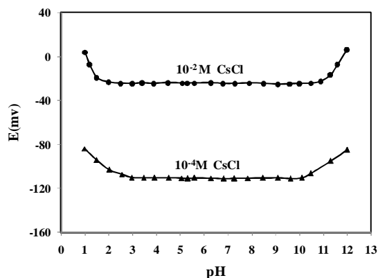
Figure 5: pH effect of the sample solutions on the potential response of \text{Cs}^+ selective electrode at 25^\circ\text{C} .
