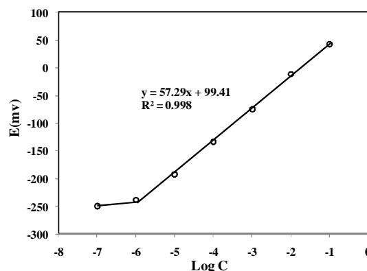
Figure 3: Calibration graph of the Cs + selective electrode based on p-IPC6 at 25°C.
