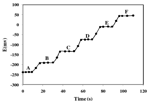
Figure 4: Dynamic response time of the Cs + selective electrode for step changes in the concentration of cesium solution: (A) 1.0 \times 10^{-6} M, (B) 1.0 \times 10^{-5} M, (C) 1.0 \times 10^{-4} M, (D) 1.0 \times 10^{-3} M, (E) 1.0 \times 10^{-2} M and (F) 1.0 \times 10^{-1} M at 25°C.
