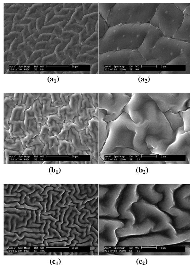
Figure 8: Scanning electron microphotographs (SEM) of cesium(I) selective PVC membrane at two magnifications: (a) membrane without ionophore that conditioned for one day, (b) membrane with ionophore that conditioned for one day and (c) membrane that conditioned for three months and used daily over the mentioned period.
