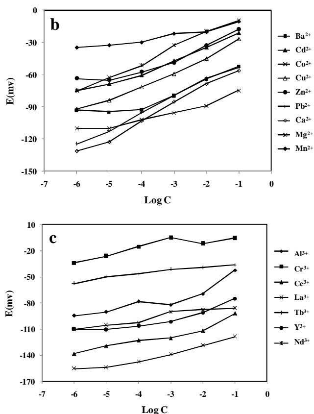
Figure 2: The potential responses of PVC membrane sensor based on p-IPC6 towards (a) monovalent, (b) bivalent and (c) trivalent cations.
