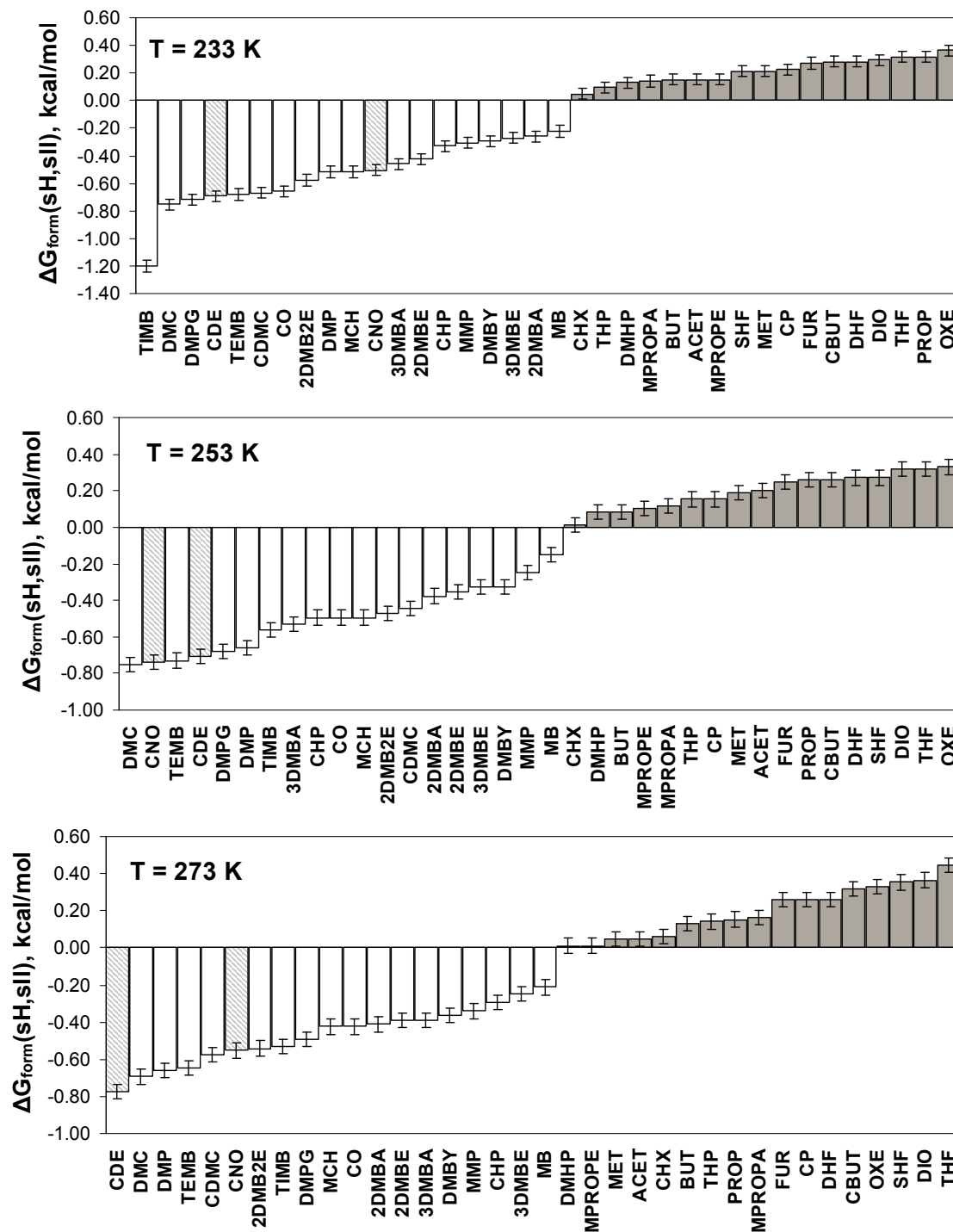
Figure 1. \Delta G_{\text{form}}(\text{sH}, \text{sII}) formation free energy for various tested promoter molecules at 1000 atm and 233 K, 253 K, and 273 K. The empty columns represent the formation free energy for enclathrated promoters known experimentally as sH clathrate formers. The solid filled columns
