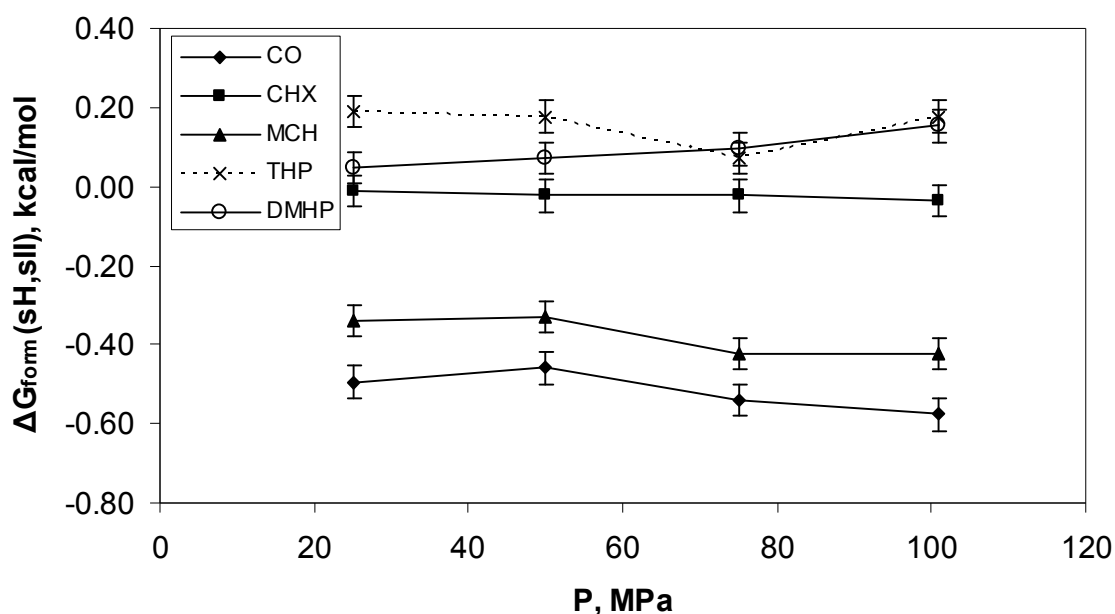
Figure 2. At 233 K formation free energy for selected tested promoter molecules at 75 MPa, 50 MPa, and 25 MPa. Errors are to two standard deviations.
