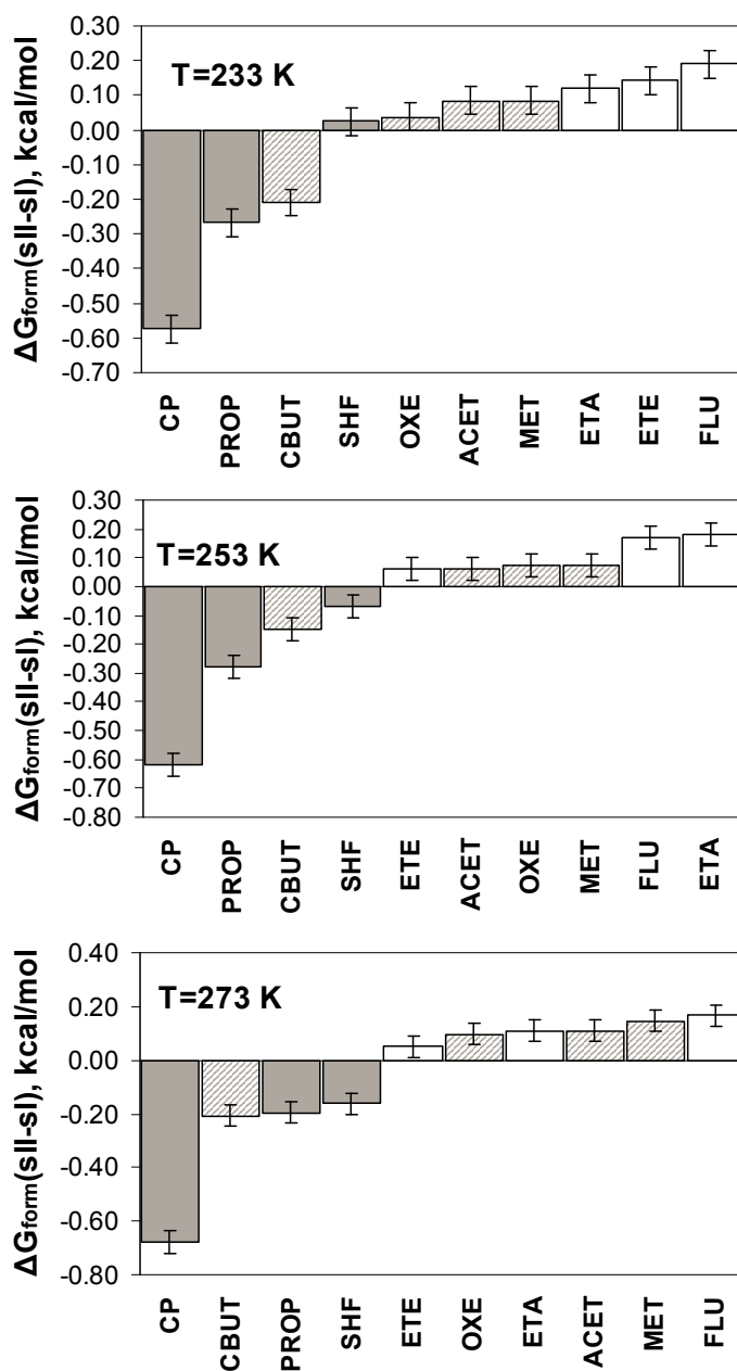
Figure 4. \Delta G_{form}(sII, sI) formation free energy for 10 selected promoter molecules at 1000 atm and 233 K, 253 K, and 273 K. The empty and solid filled columns represent \Delta G_{form}(sII, sI) for entrapped promoters known experimentally as sI and sII clathrate formers, respectively. The
