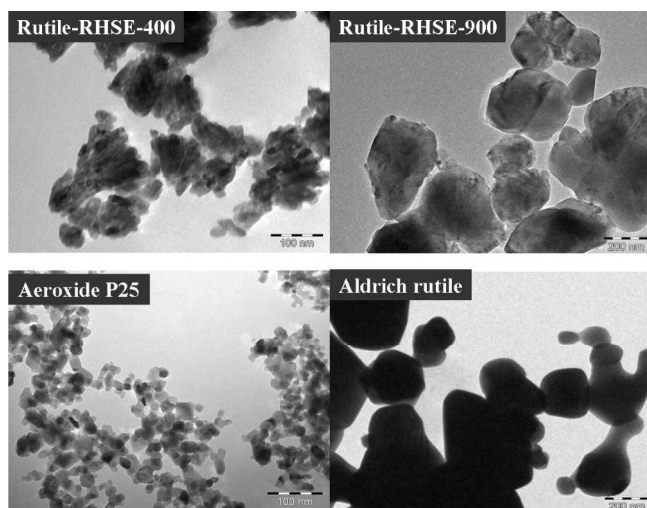
Fig. 4. TEM images of selected photocatalysts
