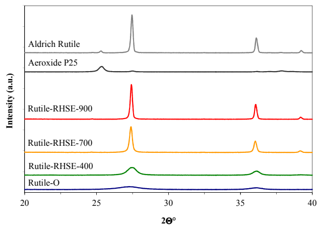
Fig. 3. XRD patterns of laboratory-made and commercial reference TiO 2 -s
