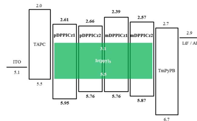
Figure 6. Energy level diagram of fabricated green OLEDs.
