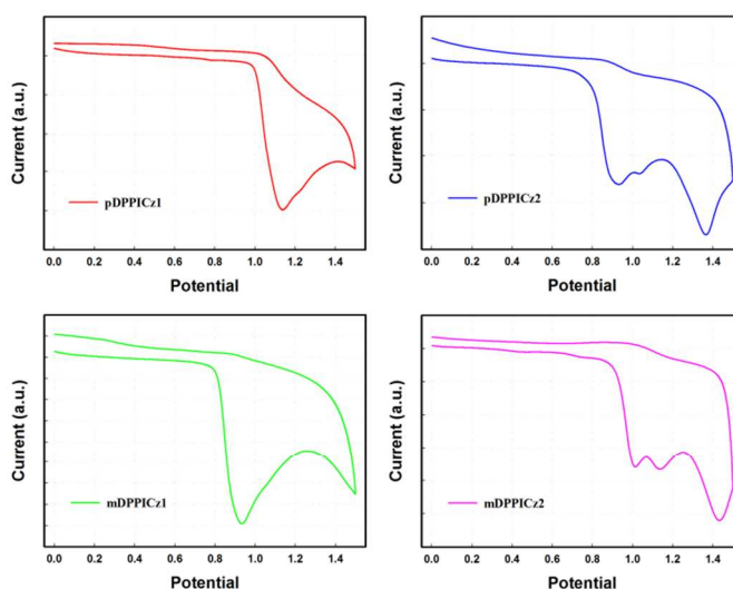
Fig. 2 CV analysis of pDPPICz1, pDPPICz2, mDPPICz1 and mDPPICz2 for oxidation potential.
