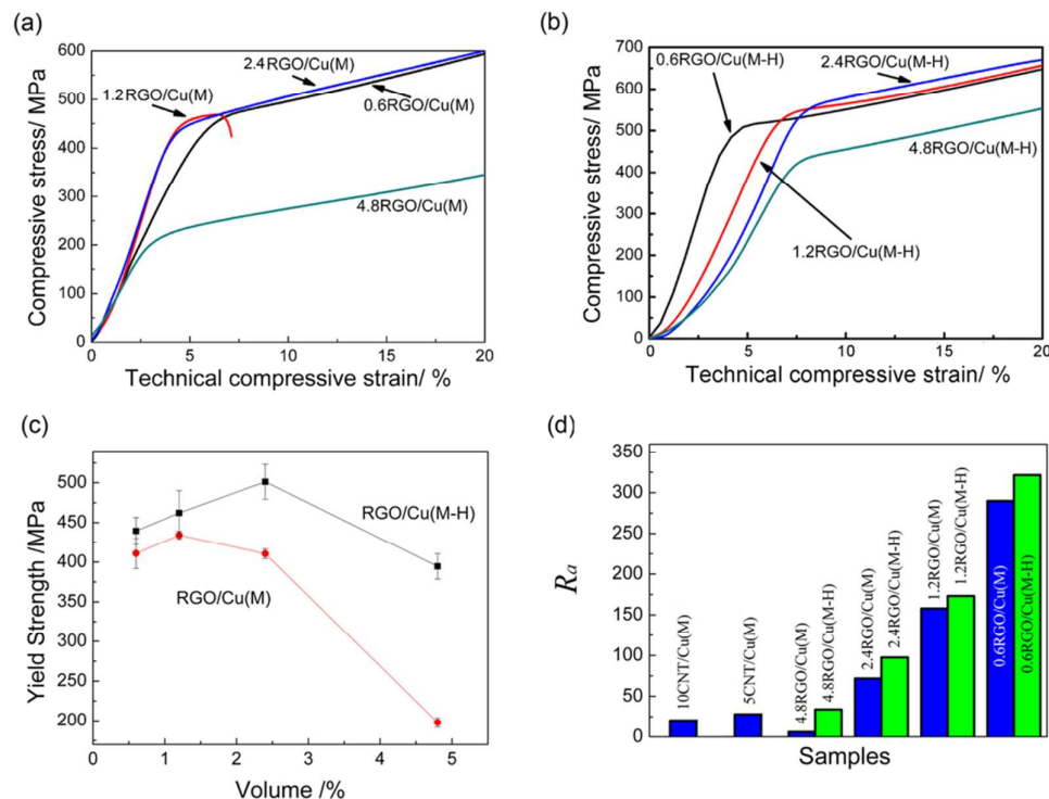
Fig. 7. Typical compressive stress-strain curves of (a) RGO/Cu(M) composites and (b) RGO/Cu(M-H); (c) comparison of compressive yield strength of the RGO/Cu composites; (d) apparent strengthening efficiencies of RGO and other reinforcements in copper matrix composites.
