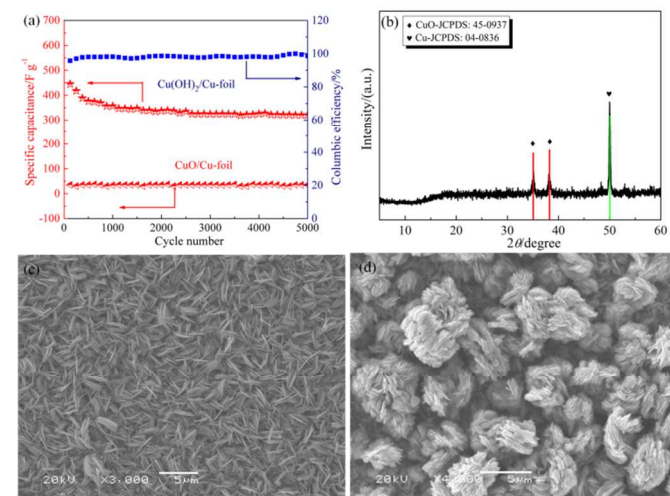
Fig. 6. Dependences of the discharge specific capacitance and the columbic efficiency on the charge/discharge cycle numbers at current density of 5 \text{ mA cm}^{-2} in 6 \text{ M KOH} electrolyte for \text{Cu}(\text{OH})_2/\text{Cu} -foil and \text{CuO}/\text{Cu} -foil electrodes (a). The XRD (b) and SEM images for \text{Cu}(\text{OH})_2/\text{Cu} -foil (c) and \text{CuO}/\text{Cu} -foil (d) electrodes after cycling.
