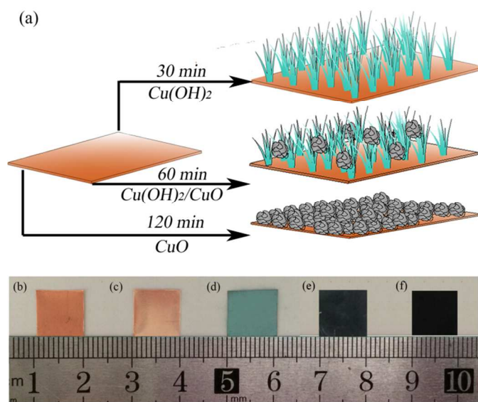
Fig. 1. Schematic diagram of Cu(OH) 2 /Cu-foil electrode (a); Photographs of Cu foil (b); The Cu foil after pretreatment (c); Cu(OH) 2 /Cu-foil electrode (d); CuO/Cu(OH) 2 /Cu-foil electrode (e); CuO/Cu-foil electrode (f).
