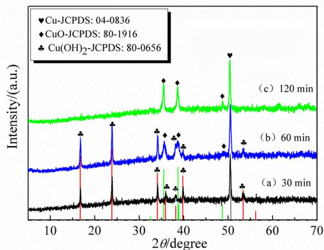
Fig. 2. XRD patterns of the Cu(OH) 2 /Cu-foil electrode, CuO/Cu(OH) 2 /Cu-foil electrode and CuO/Cu-foil electrode
