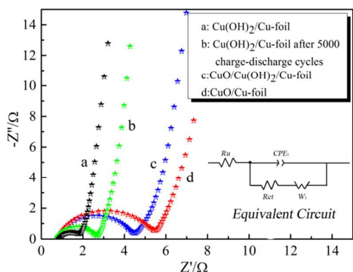
Fig. 7. EIS of the \text{Cu}(\text{OH})_2/\text{Cu} -foil electrode, \text{Cu}(\text{OH})_2/\text{Cu} -foil electrode after 5000 charge-discharge cycles, \text{CuO}/\text{Cu}(\text{OH})_2/\text{Cu} -foil electrode and \text{CuO}/\text{Cu} -foil electrode measured at open circuit potential in 6.0 \text{ mol dm}^{-3} KOH solution.
