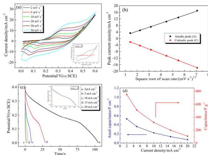
Fig. 5. CV curves of Cu(OH) 2 /Cu-foil electrode in 6 M KOH electrolyte at different scan rates (a); Voltammetric current as a function of square root of scan rate in 6 M KOH electrolyte (b); discharge curves of Cu(OH) 2 /Cu-foil electrode at different current densities in 6 M KOH electrolyte (c); variation of specific capacitance as a function of current density in 6 M KOH electrolyte (d).
