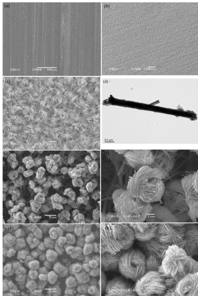
Fig. 3. SEM images and TEM images of pre-cleaned Cu foil (a), Cu(OH) 2 /Cu-foil electrode (b) (c) (d); CuO/Cu(OH) 2 /Cu-foil electrode (e) and (f); CuO/Cu-foil electrode (g) and (h).
