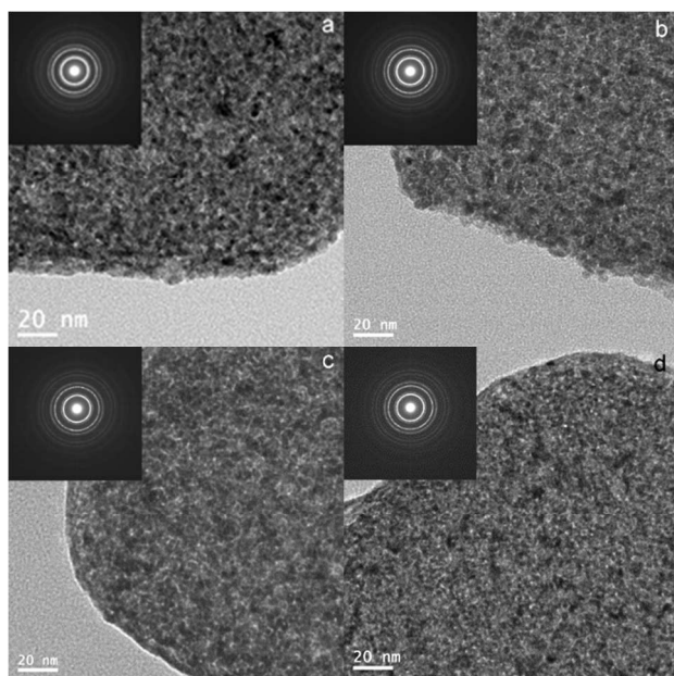
Fig. 3 TEM images and corresponding Select area diffraction patterns of 1wt% noble metal/ \text{CeO}_2 materials: Pd/ \text{CeO}_2 (a), Pt/ \text{CeO}_2 (b), Au/ \text{CeO}_2 (c) and Ag/ \text{CeO}_2 (d)
