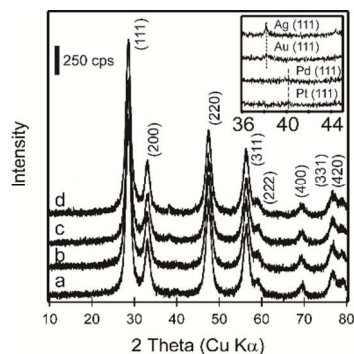
Fig. 2 XRD patterns of 1 wt% noble metal/ \text{CeO}_2 catalysts. Pd/ \text{CeO}_2 (a), Pt/ \text{CeO}_2 (b), Au/ \text{CeO}_2 (c) and Ag/ \text{CeO}_2 (d).
