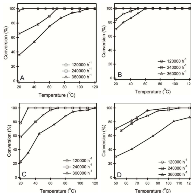
Fig. 1 Catalytic oxidation of HCHO over different noble metal/CeO 2 catalyst: Pd/CeO 2 (A), Pt/CeO 2 (B), Au/CeO 2 (C) and Ag/CeO 2 (D).
