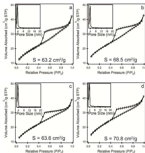
Fig. 4 \text{N}_2 desorption-adsorption isotherms and pore distributions of noble metal/ \text{CeO}_2 materials: Pd/ \text{CeO}_2 (a), Pt/ \text{CeO}_2 (b), Au/ \text{CeO}_2 (c) and Ag/ \text{CeO}_2 (d)
