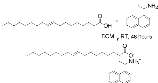
Scheme 1 Synthetic strategy used for the preparation of (NEAH) + /(OAc) - .
