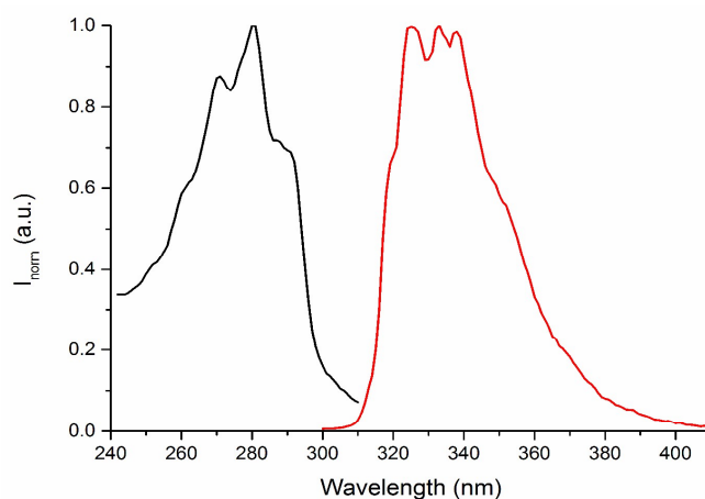
Fig. 4 Absorption (black curve) and emission (red curve) spectra of (\text{NEAH})^+ / (\text{OAc})^- emulsion in water ( (\text{NEAH})^+ / (\text{OAc})^- = 8.82 \cdot 10^{-5} \text{ M} ), \lambda_{\text{exc}} = 281 \text{ nm} .
