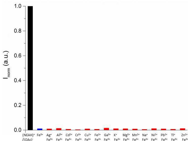
Fig. 6 Ion competition study for (NEAH) + /(OAc) - [8.82·10 -5 M] in the presence of 20 equivalents of Fe 3+ and 50 equivalents of the other metal ions in pure water at 298 K ( \lambda_{em} = 333 nm, \lambda_{exc} = 281 nm); (NEAH) + /(OAc) - (black); (NEAH) + /(OAc) - + Fe 3+ (blue); (NEAH) + /(OAc) - + metal cations + Fe 3+ (red). Emulsions of (NEAH) + /(OAc) - were diluted 1:25 times prior to the measurements.
