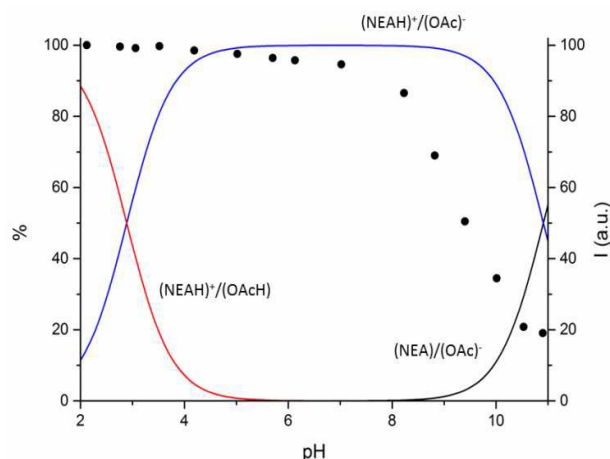
Fig. 3 Distribution diagram vs pH for (\text{NEAH})^+ / (\text{OAc})^- ( (\text{NEAH})^+ / (\text{OAc})^- = 8.82 \cdot 10^{-5} \text{ M} ) I = 0.1 \text{ M} water solution, 298 K. and (•) spectrofluorimetric emission intensities at 333 nm.
