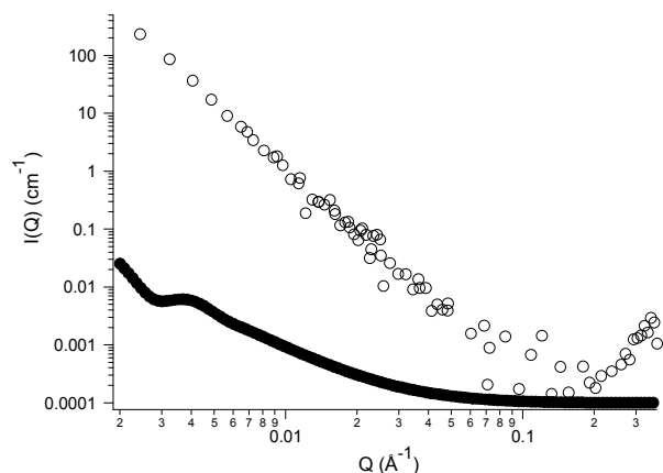
Fig. 2 SANS experimental scattered intensity (empty circles) for a sample of (\text{NEAH})^+ / (\text{OAc})^- dispersed in deuterated water (0.05 wt%, pH = 8.2), and the calculated form factor (full circles) for vesicles having a core diameter of 200 nm (polydispersity index 0.2).
