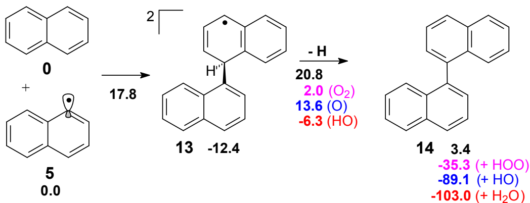
Scheme 5. Possible pathway to 1,1'-binaphthyl. The free energy level of naphthalene + naphthyl radical (which can form in several ways) has been set arbitrarily to zero (see end of section B1 and footnote 50).
