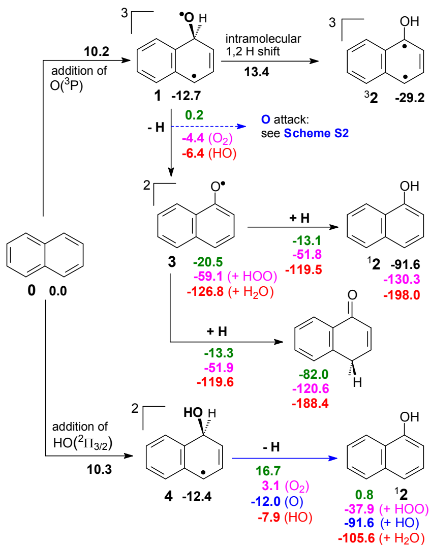
Scheme 1. Formation pathways for 1-naphthol ( C_{10}H_8O ). \Delta G values at DFT(M06-2X)/cc-pVTZ//DFT(M06-2X)/6-311G(d,p), taken with respect to the reactants level. Values originating from simple unimolecular homolytic H losses in green (taken as a reference); from bimolecular H abstractions operated by O_2 ( ^3\Sigma_g^- ) in magenta, by O ( ^3P ) in blue, and by HO ( ^2\Pi_{3/2} ) in red.
