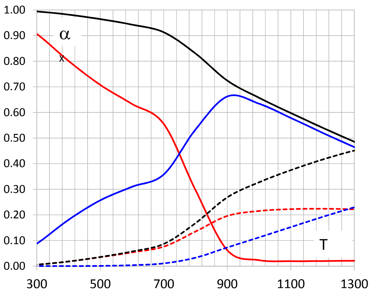
Figure 3. Branching ratios, defined for each reactive species X ( X = \text{HO}, \text{O} ) as \alpha_X = k_X / \sum_i k_{Xi} (see main text). Addition to naphthalene: continuous lines. H-abstraction from its position 1: broken lines. Red lines: X = \text{HO} . Blue lines: X = \text{O} . Black continuous line: sum of the two additions. Black dashed line: sum of the two H abstractions. At the lowest temperatures HO addition dominates, while O addition prevails beyond 800 K. Beyond 1300 K, H abstractions prevails.
