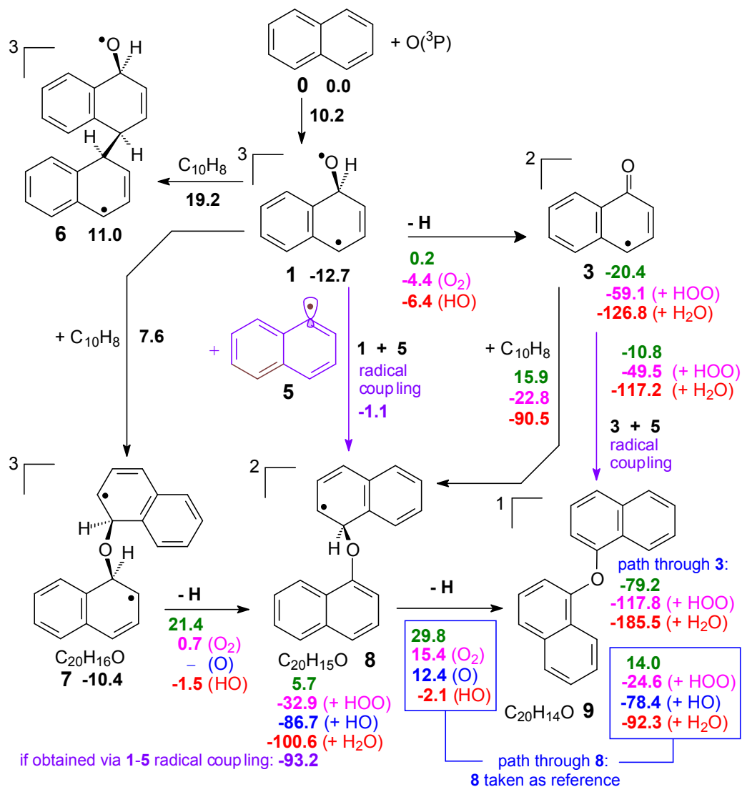
Scheme 2. Reactions of 1 and 3 with naphthalene which could cause a mass increase. \Delta G values at the DFT(M06-2X)/cc-pVTZ//DFT(M06-2X)/6-311G(d,p), taken with respect to the reactants level, unless otherwise indicated. Values originating from unimolecular homolytic H losses in green; from H abstraction operated by O ( ^3P ) in blue, by O_2 ( ^3\Sigma_g^- ) in magenta and, by HO ( ^2\Pi_{3/2} ) in red. Radical couplings are emphasized by the purple color. Boxed values are taken with respect to 8 , to avoid reporting too many figures, which inevitably originate from "mixed steps" 7-8 and 8-9 . They allow a straightforward combination of values, as desired.
