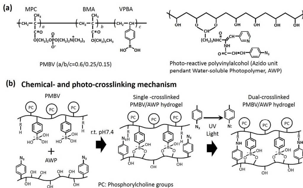
Figure 1. (a) The chemical structure of PMBV and AWP, and (b) Dual-crosslinking mechanism of PMBV/AWP hydrogel.
