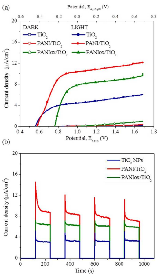
Figure 5. Photoelectrochemical characterizations for the samples: TiO_2 film (blue line), PANI/TiO_2 film (red line) and PANIox/TiO_2 (green line). (a) LSV collected with a scan rate of 10 mV/s in the dark and under illumination (AM 1.5G, 100 mW/cm 2 ) and (b) Chrono-amperometric ( I-t ) curves at an applied potential of -0.1 V vs. Ag/AgCl under illumination with 120 s light ON/OFF cycles.
