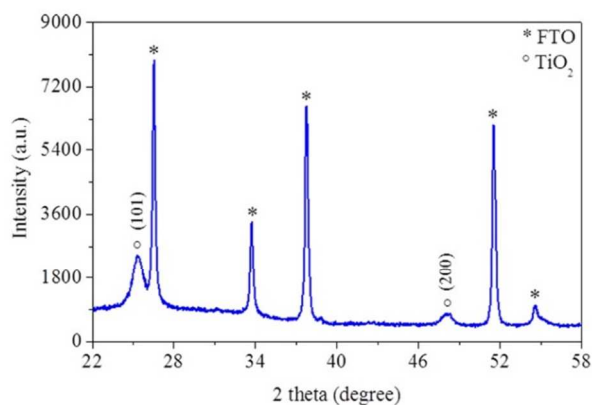
Figure 2. XRD spectrum for immobilized \text{TiO}_2 film calcined at 500^\circ\text{C} .
