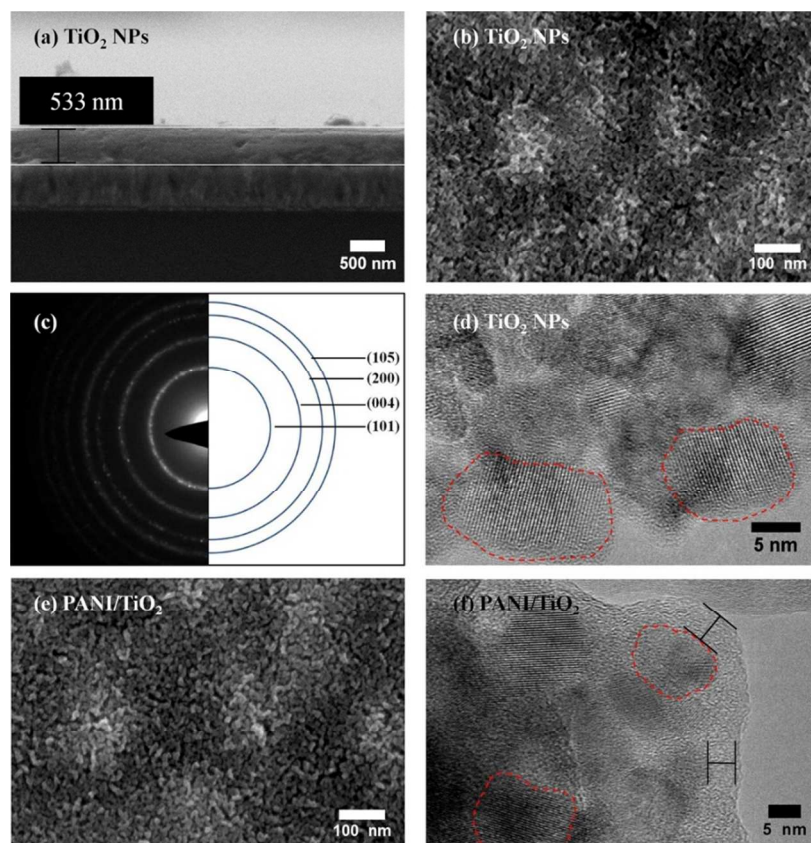
Figure 3. FESEM images of \text{TiO}_2 film in cross-section (a) and top view (b). Fragments of the film on the surface of the sample in (a) are due to sample preparation for cross-section imaging. SAED pattern of the \text{TiO}_2 sample corresponding to polycrystalline anatase \text{TiO}_2 (c). HRTEM image of the \text{TiO}_2 sample (d). Top-view FESEM image (e) and HRTEM image (f) of the PANI/ \text{TiO}_2 sample.
