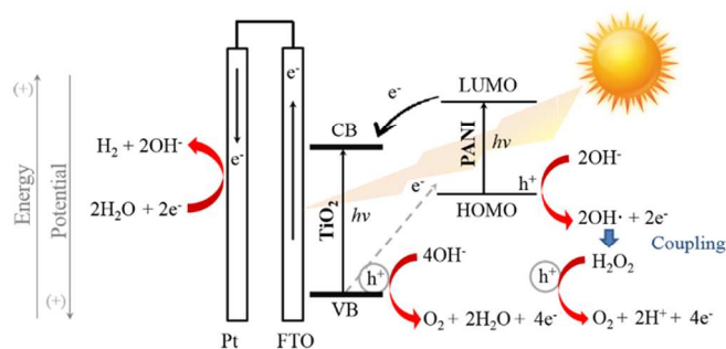
Figure 6. Mechanism of UV-Vis light absorption and charges transfer in PANI-TiO_2 composite films for the photoelectrochemical water splitting reaction in basic media.
