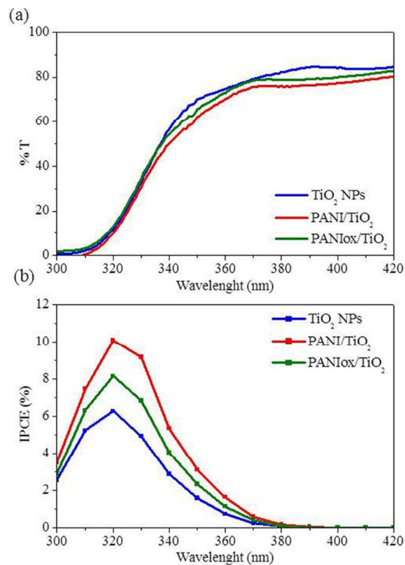
Figure 7. Optical properties for the samples: TiO 2 film (blue line), PANI/TiO 2 film (red line) and PANIox/TiO 2 (green line). (a) UV-Vis spectra recorded in transmittance mode and (b) IPCE spectra recorded by varying the wavelength of the incident light from 300 nm to 420 nm at an applied potential of 0.26 V vs. Ag/AgCl (1.23 V vs. RHE).
