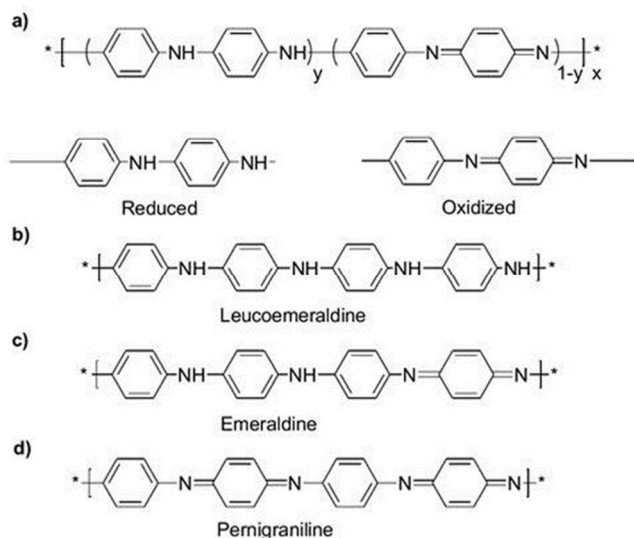
Figure 1. Generalized composition of polyanilines indicating the reduced and oxidized repeating units (a), the completely reduced polymer (b), the half-oxidized polymer (c) and the fully oxidized polymer (d). Reproduced and adapted from Ref. 37.
