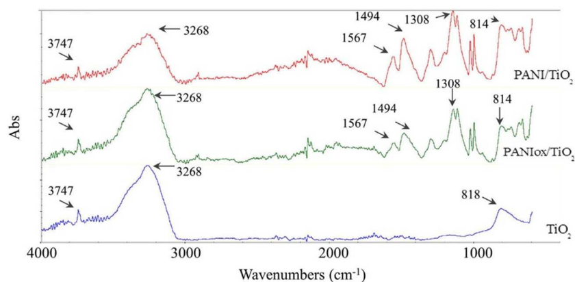
Figure 4. ATR infrared spectra of TiO 2 and PANI-TiO 2 films.
