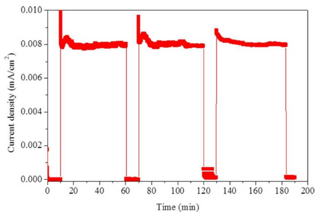
Figure 8. Photocurrent stability vs. time of PANI/TiO 2 film obtained by chrono-amperometric ( I-t ) technique at an applied potential of 0.26 V vs. Ag/AgCl (1.23 V vs. RHE) under illumination with ON/OFF cycles.
