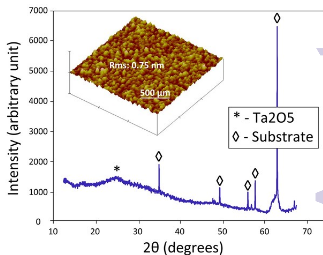
Fig. 3. X-ray diffraction (XRD) pattern of rapidly thermal annealed (RTA) Ta 2 O 5 thin film at 400 °C for 10 min in N 2 atmosphere. Inset: Topographic image characterized by atomic force microscopy (AFM).
