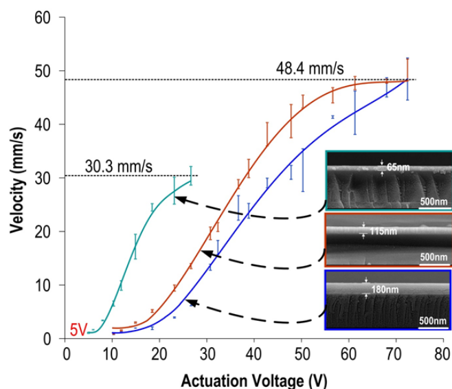
Fig. 6. Droplet transportation velocity as a function of the actuation voltage on chips with different thickness of Ta 2 O 5 layers. Insert: Scanning Electron Microscope (SEM) cross-section micrographs of different thickness of Ta 2 O 5 thin films. The velocity was an average of a droplet moving across 12 electrodes. All experiments have been repeated for three times.
