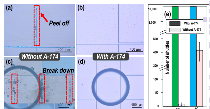
Fig. 5. Topographic images of DMF chips coated with Ta 2 O 5 and Parylene C with and without A-174 as an adhesion promoter. (a) Freshly fabricated chip without A-174. (b) Freshly fabricated chip with A-174. (c) After running droplets on chip without A-174, (d) After running droplets on chip with A-174.
