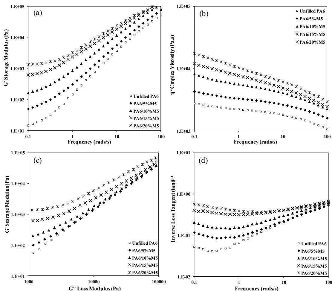
Fig. 3 – Variation in (a) storage modulus ( G' ) as a function of frequency ( \omega ); (b) complex viscosity ( \eta^* ) as a function of \omega ; (c) Cole-Cole plots ( G' versus G'' ); and (d) inverse loss tangent ( \tan \delta^{-1} ) as a function of \omega at 240°C for unfilled PA6 and PA6/M5 composites, all at 200 rpm.
