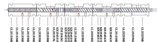
Fig. 1 Schematic of the bespoke screw profile designed to enhance the nanoparticle dispersion into a polymer matrix. KB=Kneading Blocks, GL=Conveying elements; Z=Mixing elements; L= Reverse flow effect, R= forward flow effect.
