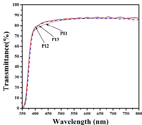
Fig. 4 UV–vis transmission spectra of PI films (film thickness: 10 \mu\text{m} )
