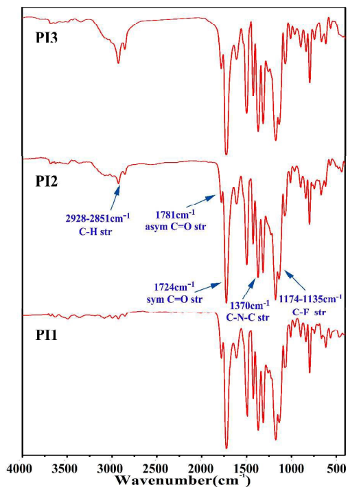
Fig. 3 Thin film FT-IR spectrum of PIs
