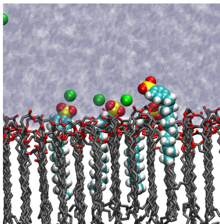
Fig. 1 Molecular dynamics simulations predict that sodium dodecylbenzene sulphonate surfactant molecules embed themselves in a tristearin bilayer, packing commensurate with the hexagonally packed lattice formed by the acyl tails of tristearin.
