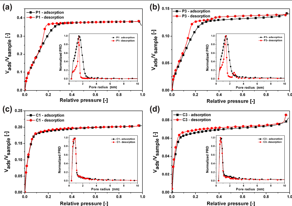
Fig. 12 Toluene adsorption-desorption isotherms at 294 K of (a-b) Pluronic and (c-d) CTAB-templated silica coatings irradiated with Xe + ions with fluences of 10^{15} cm -2 and 10^{16} cm -2 , respectively, measured by ellipsometric porosimetry. The insets show the normalized pore radius distributions.
