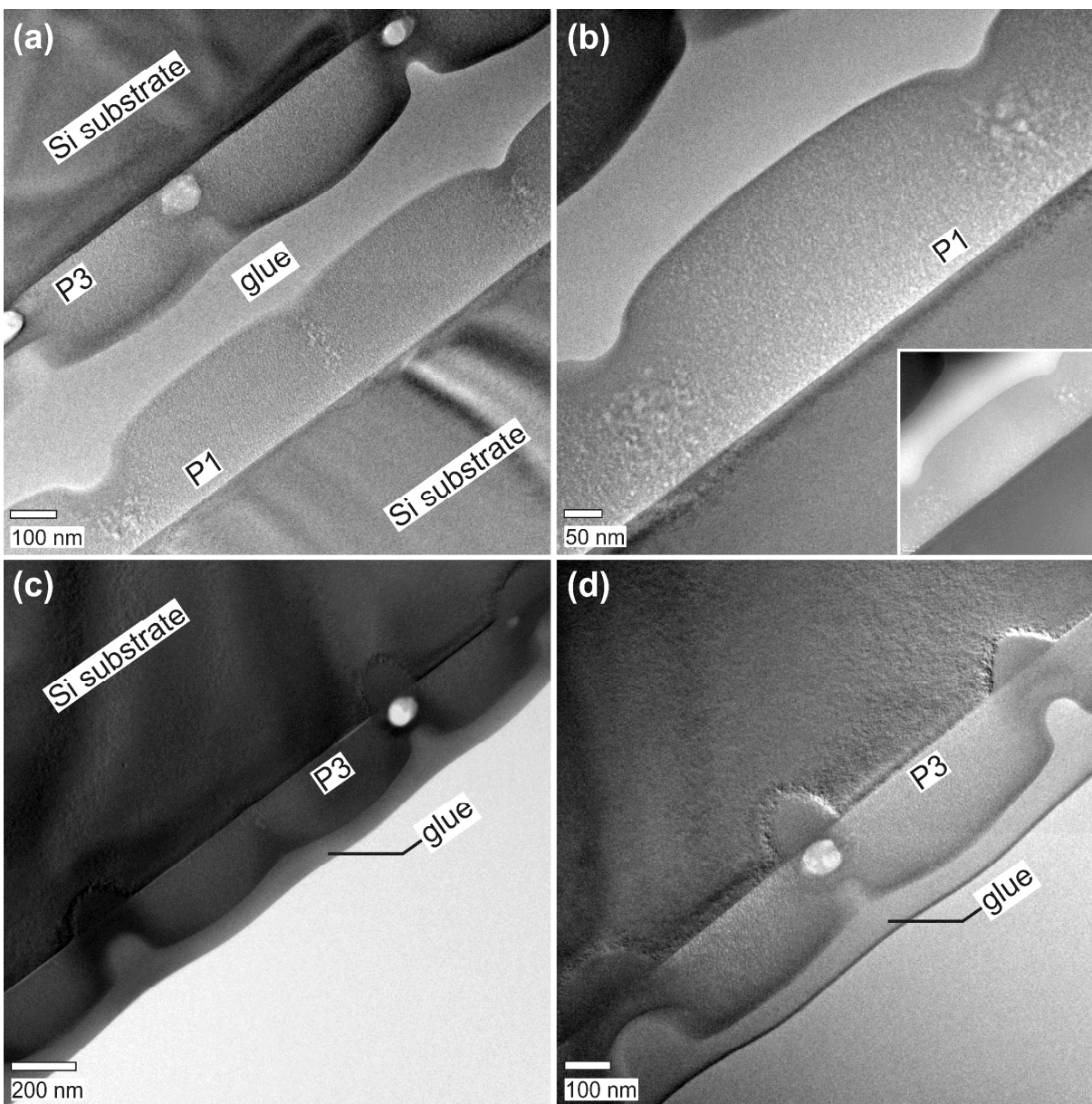
Fig. 8 Cross-sectional HRTEM images of Pluronic-templated silica coatings irradiated with Xe^+ fluences of (a, b) 10^{15} \text{ cm}^{-2} (denoted as "P1") and (a, c, d) 10^{16} \text{ cm}^{-2} ("P3") through the particulate mask. The inset shows the EELS image of the same area as in (b). Note that the plane of cross section does not necessarily intersect the axis of the porous columns.
