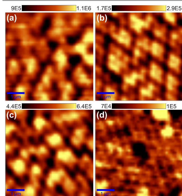
Fig. 10 Confocal fluorescent images of (a-b) Pluronic and (c-d) CTAB-templated silica coatings irradiated with \text{Xe}^+ ions to fluences of 10^{15} \text{ cm}^{-2} and 10^{16} \text{ cm}^{-2} , respectively. The upper scale bars show the collected CCD counts.
