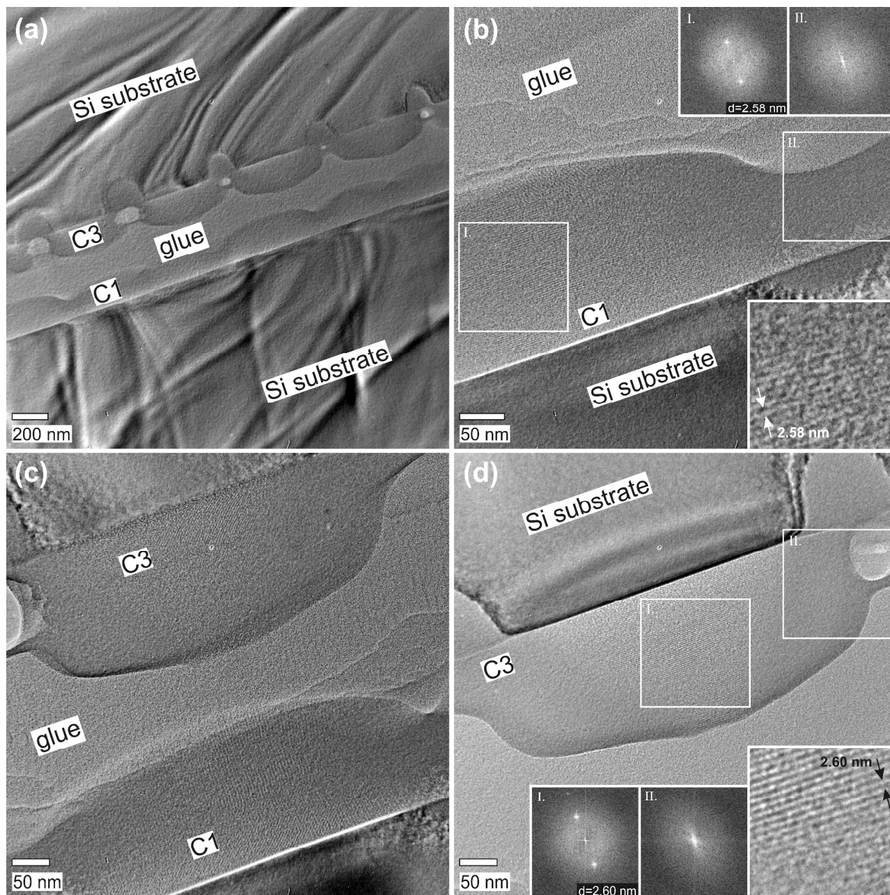
Fig. 9 Cross-sectional HRTEM images of CTAB-templated silica coatings irradiated with \text{Xe}^+ fluences of (a, b, c) 10^{15} \text{ cm}^{-2} (denoted as “C1”) and (a, c, d) 10^{16} \text{ cm}^{-2} (“C3”). The insets in (b) and (d) show the magnified transition area of the same image between the intact, ordered and the destroyed, densified pore structure, and the FFTs of marked regions.
