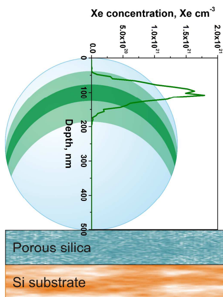
Fig. 1 Schematic view of 200 keV Xe + ion bombardment with the fluence of 10 16 cm -2 through a silica sphere with diameter of 500 nm. The solid line shows the ion profile resulted by SRIM simulations.
