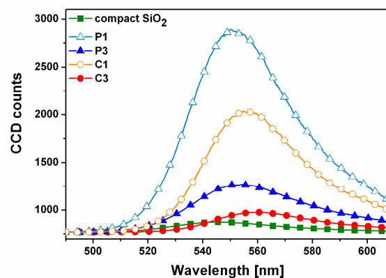
Fig. 11 Averaged confocal fluorescent spectra measured on Pluronic- (denoted as "P1" and "P3") and CTAB-templated ("C1" and "C3") silica coatings irradiated with ion fluences of 10^{15} cm -2 ("P1", "C1") and 10^{16} cm -2 ("P1", "C1") and impregnated with 10^{-4} M aqueous Rhodamine 6G solution. A compact silica sol-gel coating was prepared without any molecular template and it was immersed into the same solution for comparison.
