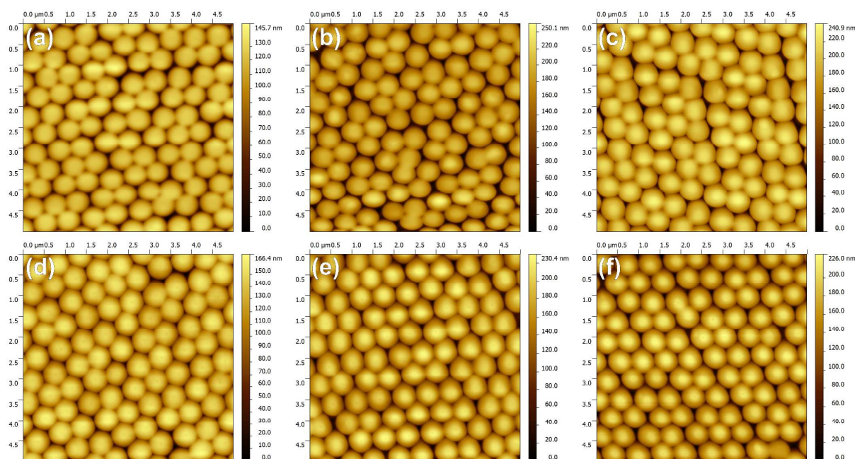
Fig. 5 Columnar surface morphology measured by AFM on (a-c) Pluronic and (d-f) CTAB-templated silica coatings irradiated with Xe + ions through LB mask of silica particles with fluences of 0.1, 0.5, and 1 × 10 16 cm -2 , respectively. Please note that the maximum value of z-scale depends on the largest distance between two columns and on the actual tip geometry.
