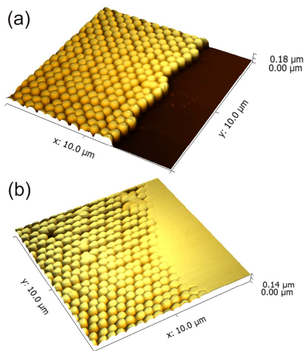
Fig. 4 3D representations of surface morphology measured by AFM on Pluronic-templated silica coatings after ion irradiation with fluences of (a) 10 15 cm -2 and (b) 10 16 cm -2 , respectively. The measurements were carried out (a) where the edge of the particulate LB mask was located and (b) at the border of irradiated and unirradiated regions of the LB film (the right side was masked by an additional metal plate).
