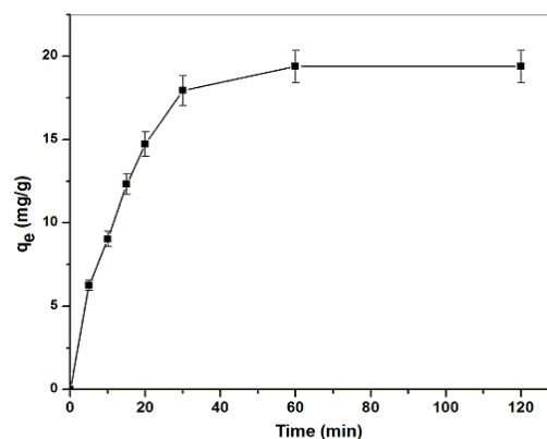
Fig. 8 Time dependence of Cd(II) adsorption capacity on DEAMTPP@Fe 3 O 4 MNPs.
