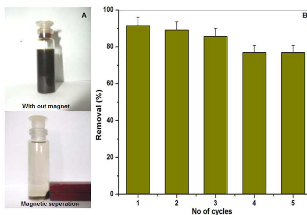
Fig. 12 (A) magnetic separation and (B) Recycling efficiency of DEAMTPP@Fe 3 O 4 MNPs for Cd(II) adsorption during cyclic experiments (MNP concentration: 0.1 g/L at pH 6.0).
