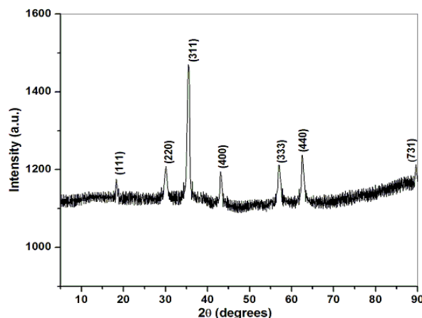
Fig. 1 PXRD pattern of DEAMTPP@Fe 3 O 4 MNPs.
