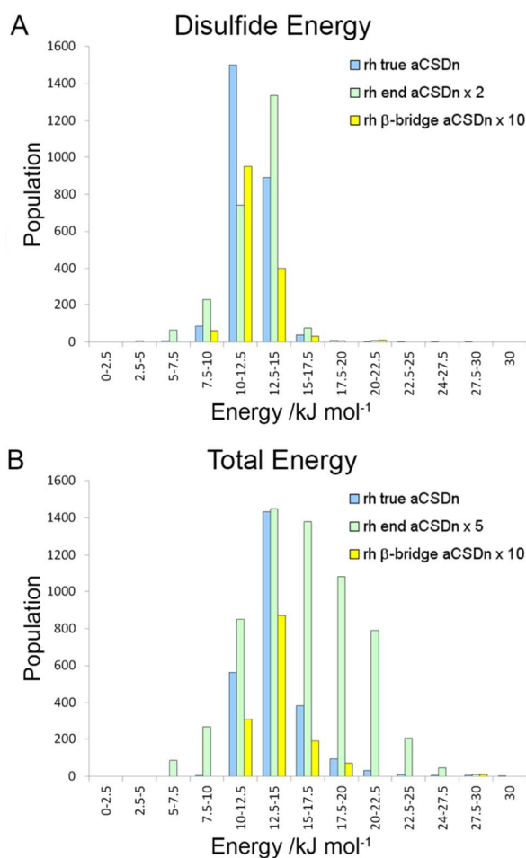
Figure 7. Distribution of torsional energies for right-handed disulfides in aCSDn motifs. A The disulfide torsional energy (DTE) distribution. I.e. the strain in \chi_2, \chi_3 and \chi_2' . B The total torsional energy (TTE) distribution. I.e. the strain in \chi_1, \chi_2, \chi_3, \chi_2' and \chi_1' . The populations for end- and \beta -bridge aCSDns have been scaled, as described in the legend, to allow easy comparison on the same set of axes.
