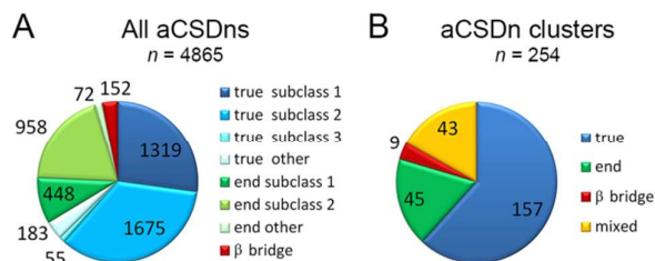
Figure 3. A The distribution of the aCSDns in our dataset amongst the three possible sub-motifs and their subclasses. B The distribution of non-homologous aCSDns clusters in our dataset amongst the sub-motifs. The “mixed” group includes all clusters where there is heterogeneity in the sub-motifs observed.
