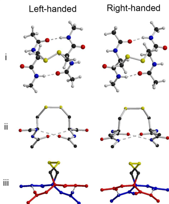
Figure 8. Optimised geometries for the aCSDn model compound. Compounds with a left-handed staple disulfide induce a left-handed twist in the sheet, whereas those with a right-handed staple disulfide induce a right-handed sheet twist. i View looking down onto the face of the sheet. ii View from the side looking along the strands. Atom sizes have been reduced and hydrogen atoms removed to improve clarity. iii View from the side across the strands. The chains have been given different colours to emphasise the sheet twist. Figure prepared using Molscript 28 and Raster3D 29 .
