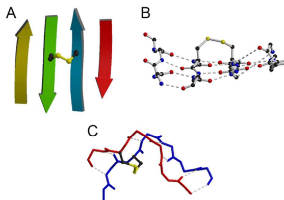
Figure 1. A and B A representative disulfide in an aCSDn motif (true-aCSDn-2) from human amyloid serum P component: PDB 2a3y A Cys 36 to Cys 95. Note: the introduction of the disulfide does not cause noticeable buckling of the \beta -sheet (only the usual sheet twist is observed) and the hydrogen bonds are locally flat. C A representative subclass 3 true-aCSDn (disulfide immediately adjacent to an A-bent bulge) from the surface active protein hydrophobin: PDB 1r2m A Cys 14 to Cys 26. Figure prepared using Molscript ® and Raster3D ™ .
