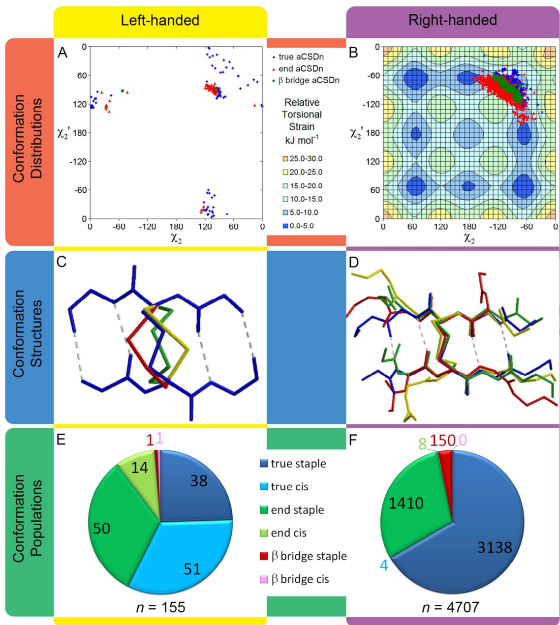
Figure 6. Disulfide conformations adopted by aCSDn motifs showing the homogeneity of right-handed aCSDn conformations and the heterogeneity of left-handed structures. A and B show the \chi_2 and \chi_2' dihedral angles adopted by left- and right-handed aCSDns, respectively. Conformations of right-handed disulfides with 85^\circ \leq \chi_3 \leq 115^\circ (representing > 95% of right-handed aCSDns) are superimposed on a contour plot of the potential energy surface (PES) for torsion around \chi_2 and \chi_2' ( \chi_3 = 100^\circ ). In most cases these disulfides are associated with medium-energy (turquoise) regions of the surface. Due to the much wider range of \chi_3 dihedral angles seen for left-handed conformations, it is not instructive to superimpose these conformations on a PES plot for a single value of \chi_3 , see Methods . In C and D representative structures of the various disulfide conformations and sub-motifs adopted by aCSDns are superimposed. C Disulfides with left-handed conformations contrasted with a right-handed staple shown in blue (PDB: 1rgx Cys 35 to Cys 88) (a single representative backbone has been used to improve clarity): left-handed staple (green, PDB: 2bba Cys 61 to Cys 184), left-handed cis from upper left of map A (red, PDB: 3flp Cys 37 to Cys 103), left-handed cis from lower right of map A (yellow, PDB: 2ny0 Cys 1130 to Cys 1159). D Disulfides with right handed conformations: normal true-aCSDn (blue, PDB: 1rgx Cys 35 to Cys 88), true-aCSDn adjacent to an A-bent bulge (green, PDB: 1du5 Cys 51 to Cys 61), end-aCSDn (yellow, PDB: 2fkl Cys 133 to Cys 187), \beta -bridge-aCSDn (red, PDB: 1ivy, Cys 60 to Cys 334). All structures are seen to adopt very similar right-handed staple conformations. Parts C and D prepared using Molscript TM and Raster3D TM . E and F show relative populations left- and right-handed aCSDns in our dataset and their distribution amongst the various aCSDns sub-motifs and disulfide bond conformations.
