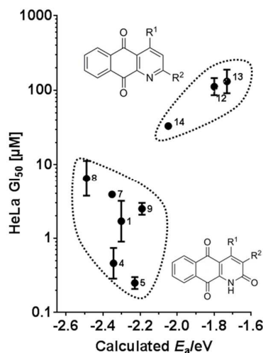
Fig. 6 Interdependency of antiproliferative activity of tested compounds with their intrinsic electrochemical properties. Correlation of calculated electron affinities and measured GI_{50} values in HeLa cells for pyridine and 2-pyridone series.
