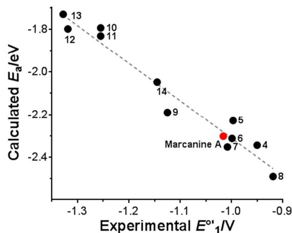
Fig. 4 Correlation of experimental formal potentials E_1^{o'} with calculated adiabatic electron affinities E_a . E_a = -1.75 * E_1^{o'} - 4.06 ; R^2 = 0.96 .
