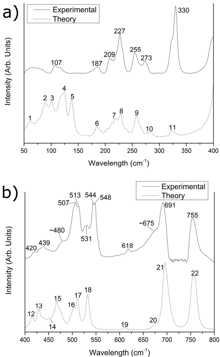
Figure 1: Experimental (solid line) and simulated (dashed line) far-IR spectra of the [(\text{PPh}_3\text{Au})_3\text{O}]\text{BF}_4 cluster in the (a) 50–400 \text{cm}^{-1} region and (b) 400–800 \text{cm}^{-1} region. The experimental data was recorded at (a) pure sample and (b) a 1:3 sample/PE dilution by mass. The simulated spectrum has been corrected by Eq 1.
