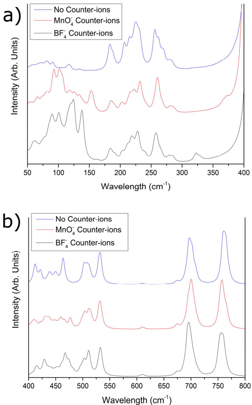
Figure 3: Comparison between theoretically calculated far-IR spectra of the tris(triphenylphosphinegold)oxonium salts with no counter-ions present (blue), MnO 4 counter-ions present (red), and BF 4 counter-ions present (black), in the (a) 50–400 cm -1 region and (b) 400–800 cm -1 region. The simulated spectra have been corrected by Eq 1.
