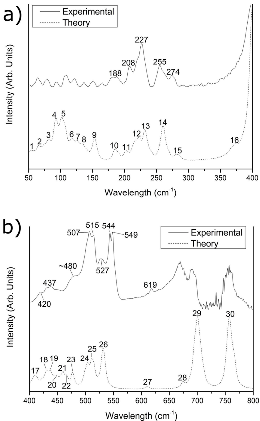
Figure 2: Experimental (solid line) and simulated (dashed line) far-IR spectra of the [(\text{PPh}_3\text{Au})_3\text{O}]\text{MnO}_4 cluster in the (a) 50–400 cm -1 region and (b) 400–800 cm -1 region. The experimental data was recorded at (a) a 1:1 sample/PE dilution by mass and (b) a 1:3 dilution by mass. The simulated spectrum has been corrected by Eq 1.
