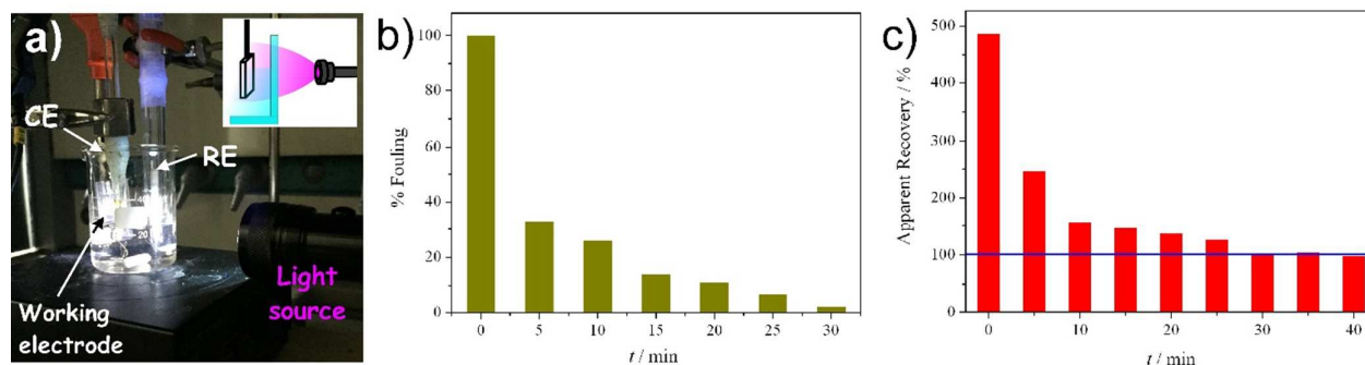
Figure 4. Scheme of the on site experiment (a). Study of fouling/recovery (b) directly in the electrolyte solution and (c) Apparent Recovery for 1 \mu M of dopamine after performing the cleaning procedure in situ with the TORCH.
