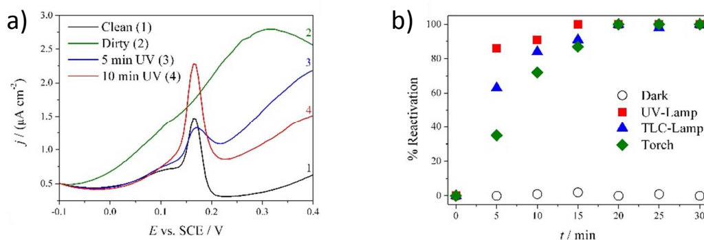
Figure 3. a) Differential pulse voltammograms acquired during the fouling/cleaning procedure: in the absence of dopamine (curve 1, AgNPs peak at 0.165 V); after fouling (curve 2, dopamine peak at 0.3 V), after UV cleaning at different time (curve 3-4). b) % Reactivation values obtained for irradiation with the three lamps and in the dark.
