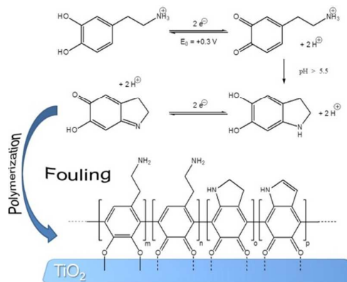
Figure 2. Schematic representation of dopamine fouling 28,29
