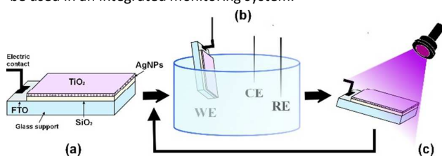
Figure 1. Schematic representation of the device (a), electrochemical cell (b) and cleaning under UV (c).
