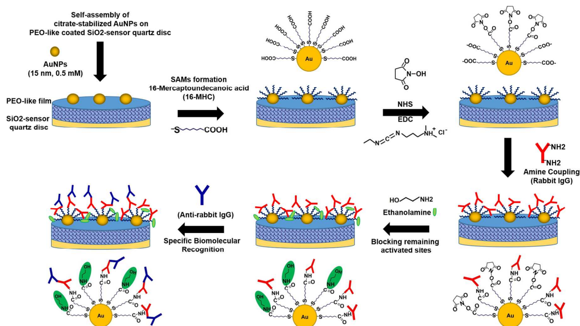
Figure 4. Schematic representation of the successive steps occurring during the immobilization of Au NPs on PEO-like coated QCM quartz, the online surface functionalization and immunodetection.
