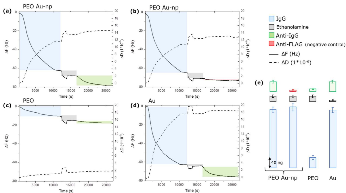
Figure 5. QCM results showing the online functionalization of Au NPs nanostructured PEO-like coated samples ( A and B ), PEO-like coating only ( C ) and flat gold ( D ) samples with rabbit IgGs, followed by specific recognition with anti-rabbit IgGs on Q1, Q3 and Q4. A solution of anti-FLAG antibodies was injected on sample Q2 as a negative control. \Delta F represents the frequency shift and \Delta D , the variation of the dissipation frequency. The immobilized mass for each step was calculated using the Sauerbrey equation and reported in ( E ).
