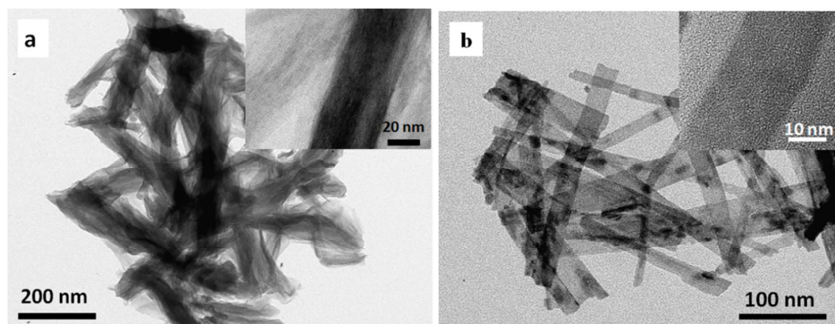
Fig. 3 TEM and HRTEM images (in the inset) of representative \text{TiO}_2 NFs synthesized at 80 °C for 24 h (a) and at 100 °C for 72 h (b).
