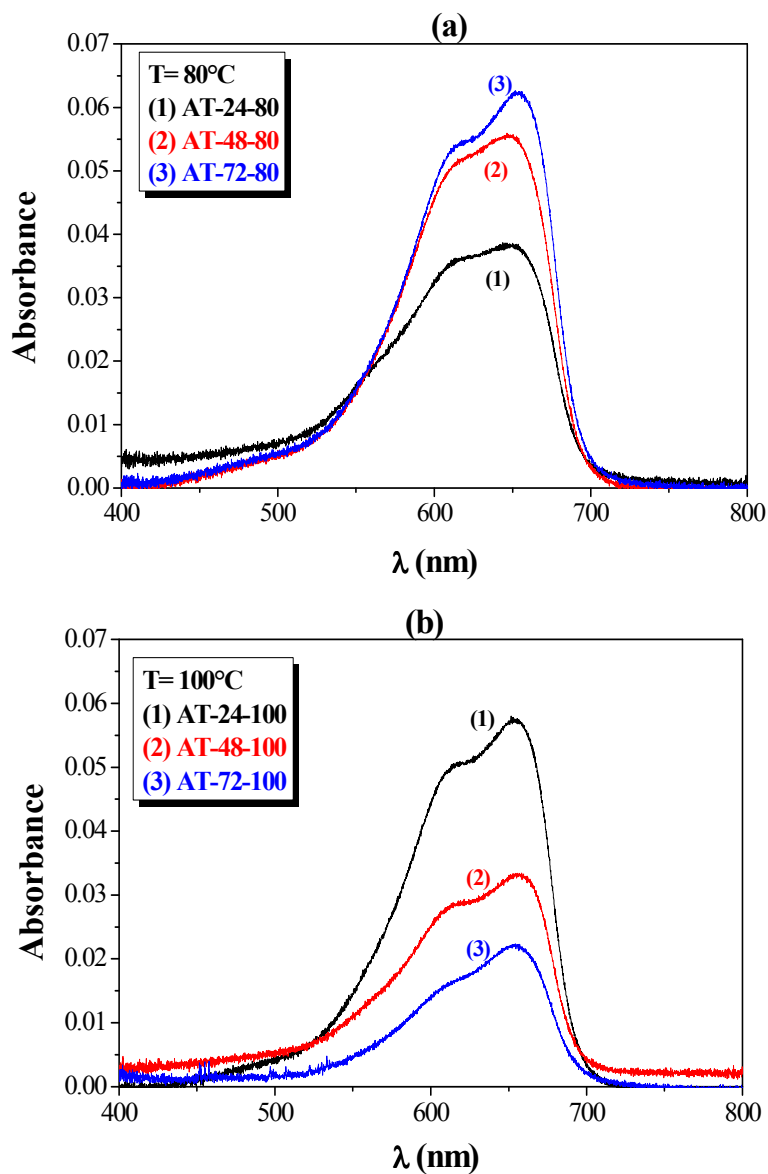
Fig. 7 Variation of the dye absorption spectra after a UV radiation exposition of 22 h in presence of \text{TiO}_2/\text{Ti} films produced at 80^\circ\text{C} (a) and 100^\circ\text{C} (b) for different heating times.
