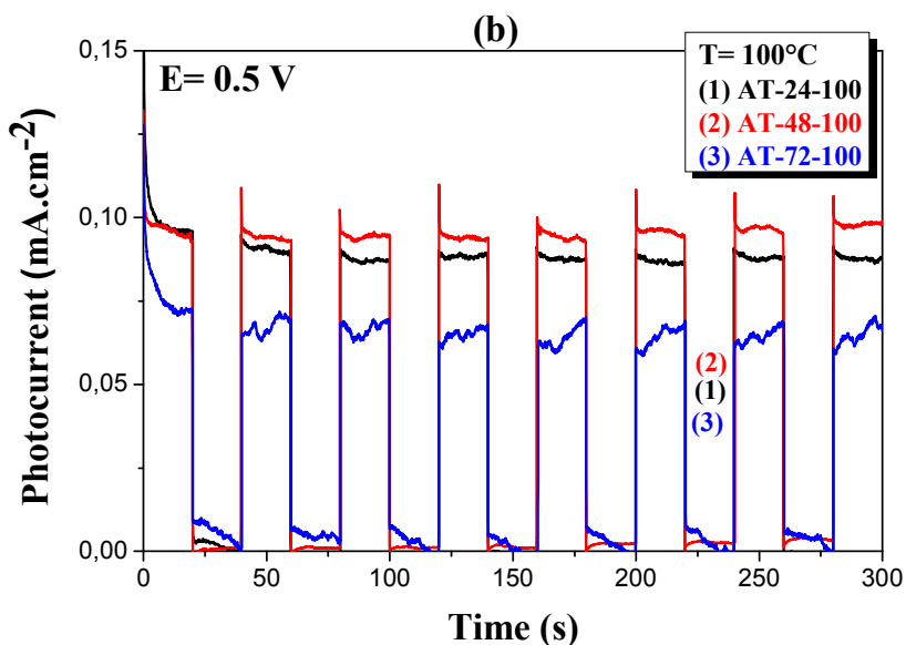
Fig. 10 Photocurrent responses in the Na 2 SO 4 aqueous solution (0.5 M, pH = 7) of TiO 2 /Ti films produced at 80 (a) and 100 °C(b) for different heating times, with a bias E = 0.5 V vs SCE.
