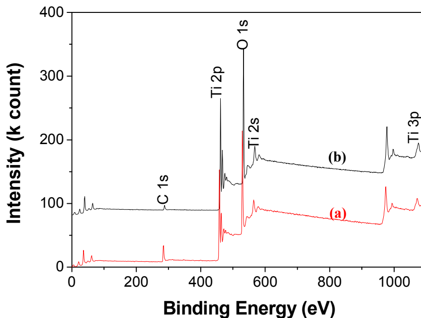
Fig. 4 Low resolution XPS spectra of \text{TiO}_2/\text{Ti} nanostructures synthesized at 80 °C for 24 h (a) and at 100 °C for 72 h (b).
