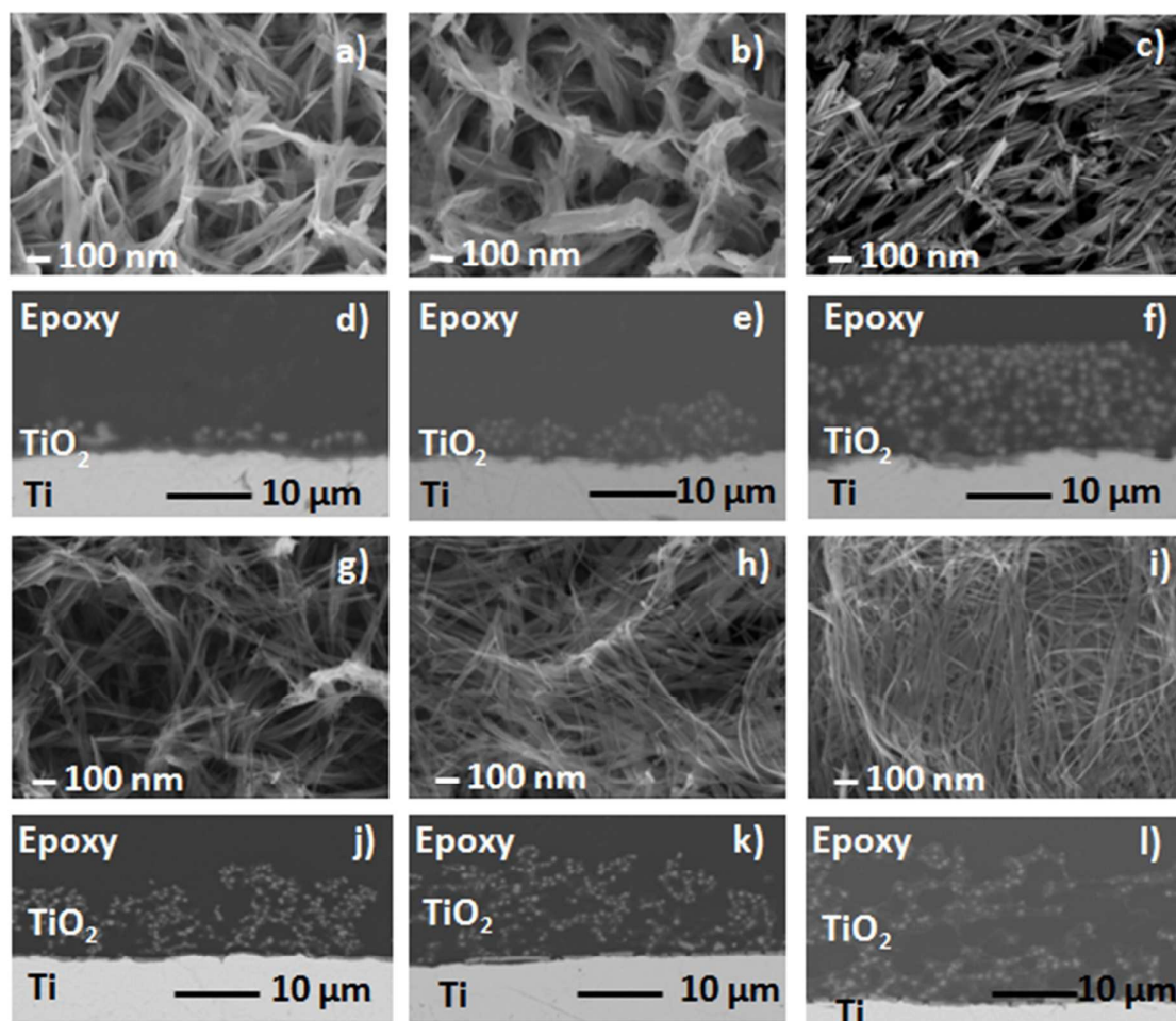
Fig. 2 Top (a, b, c) and cross section (d, e, f) views of the \text{TiO}_2/\text{Ti} nanostructures synthesized by hydrothermal oxidation of Ti sheets at 80 °C for 24, 48 and 72h, respectively, and their analogous (g, h, i) and (j, k, l) for the nanostructures obtained at 100°C for the same heating times.
