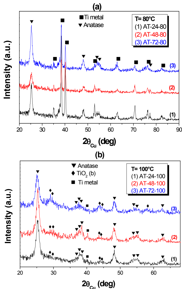
Fig.1 XRD patterns of the synthesized TiO_2 nanostructures (a) at 80^\circ C and (b) at 100^\circ C for different heating time.
