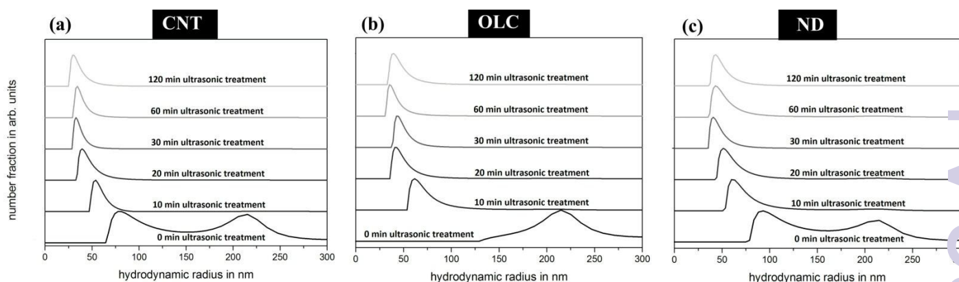
Figure 2: DLS data of a) CNT, b) OLC, and c) ND in ethylene glycol after different times of ultrasonic treatment. The spectrum of at 0 min is equal to a pre-treatment of 5 min in the homogenizer to break up the largest agglomerates.
