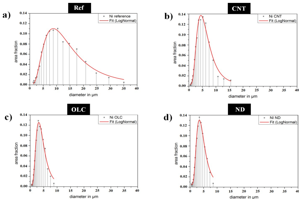
Figure 8: Grain size distribution of a) unreinforced Nickel reference, b) Ni CNT, c) Ni OLC, and d) Ni ND composites. A LogNormal fit is performed to calculate the mean grain size and the fitted curves are plotted as solid lines (red).
