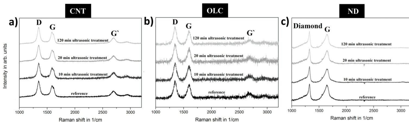
Figure 4: Raman spectra of CNT (a), OLC (b) and ND (c) on a silicon wafer as a function of the time spent in the ultrasonic bath in the solvent ethylene glycol.
