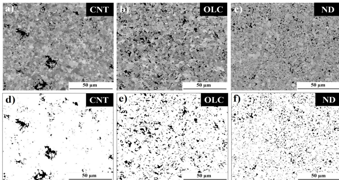
Figure 6: SEM pictures of a) CNT-, b) OLC-, and c) ND- nickel matrix composites after polishing at the top surface. The uniaxial pressure is applied at the bottom and top surface of the samples. The pictures are binarized for d) CNT-, e) OLC-, and f) ND- nickel matrix composites to enable a better qualitative comparison. The agglomerate sizes decrease significantly and the distribution of the particles becomes more homogenous from a) to c) or rather d) to f).
