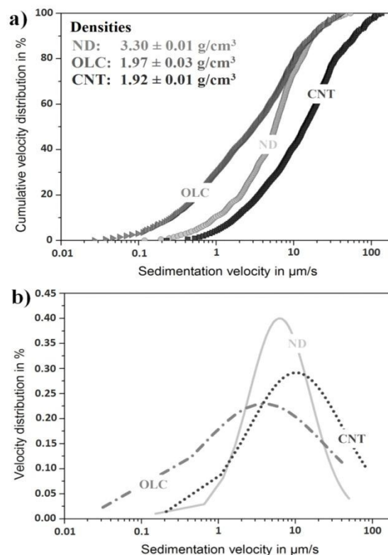
Figure 3: Sedimentation analysis of CNT, OLC, and ND dispersion in ethylene glycol showing a) the sedimentation velocity of the particles as cumulative plot (including particle densities) and b) the fitted data using a log-normal function.
