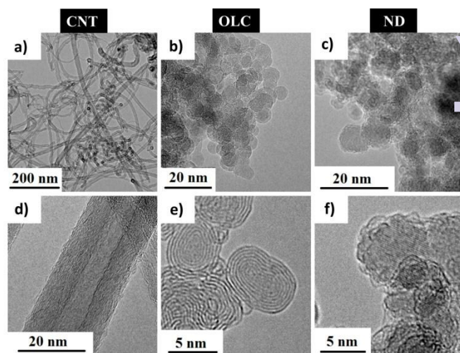
Figure 1: TEM images of MWCNT (a, d), OLC (b, e), and ND (c, f) nanoparticles.
