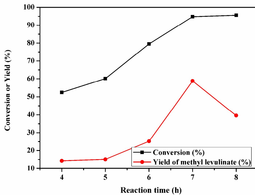
Fig. 5 The effect of reaction time on alcoholysis of cellulose. Reaction conditions: 100 mg of cellulose, 0.07 mmol of (C_{16}TA)H_3P_2W_{18}O_{62} , 8 mL methanol at 160 °C.
