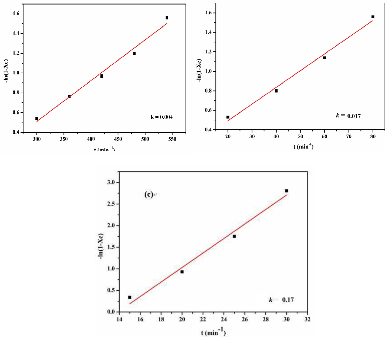
Fig.7 Kinetic behavior for polysaccharide to glucose over (C_{16}TA)H_5P_2W_{18}O_{62} . (a) cellulose; (b) starch; and (c) cellobiose.
