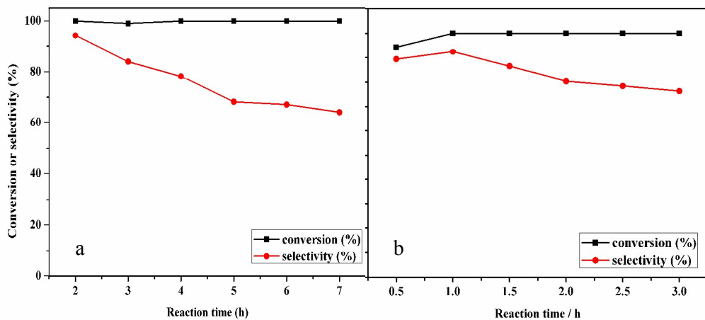
Fig. 4 The influence of reaction time and temperature on starch (a) and cellobiose (b) dehydration. Reaction conditions: 0.1g of substrates, 0.08 mmol of (C_{16}TA)H_5P_2W_{18}O_{62} , 5 ml of water at 120 °C for starch and 0.03 mmol of (C_{16}TA)H_5P_2W_{18}O_{62} , 100 °C for cellobiose, respectively
