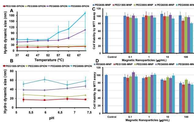
Fig. 2. Stability measurements of PEG-SPIONs (A) vs temperature in PBS buffer and (B) vs pH in water. Cytotoxicity of the PEG-SPIONs by the MTT assay of MG-63 cells treated for 24 h (C) and 72 h (D) at different concentrations.
